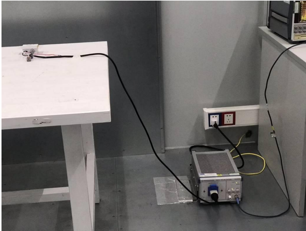
Radiated emission test 30MHz – 1GHz
