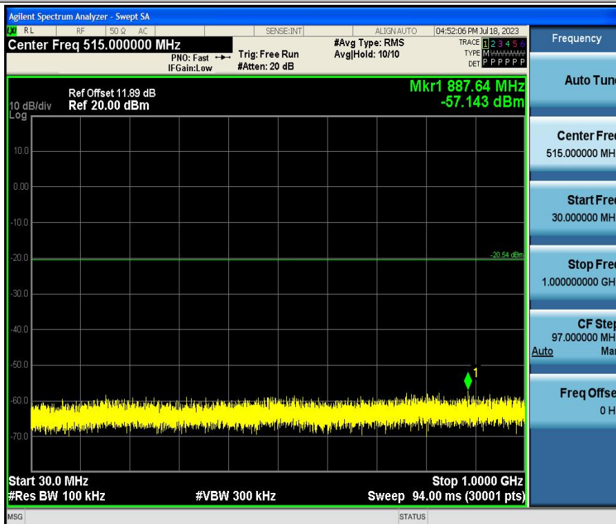
BLE_1M-Ant1-2402-0~Reference
