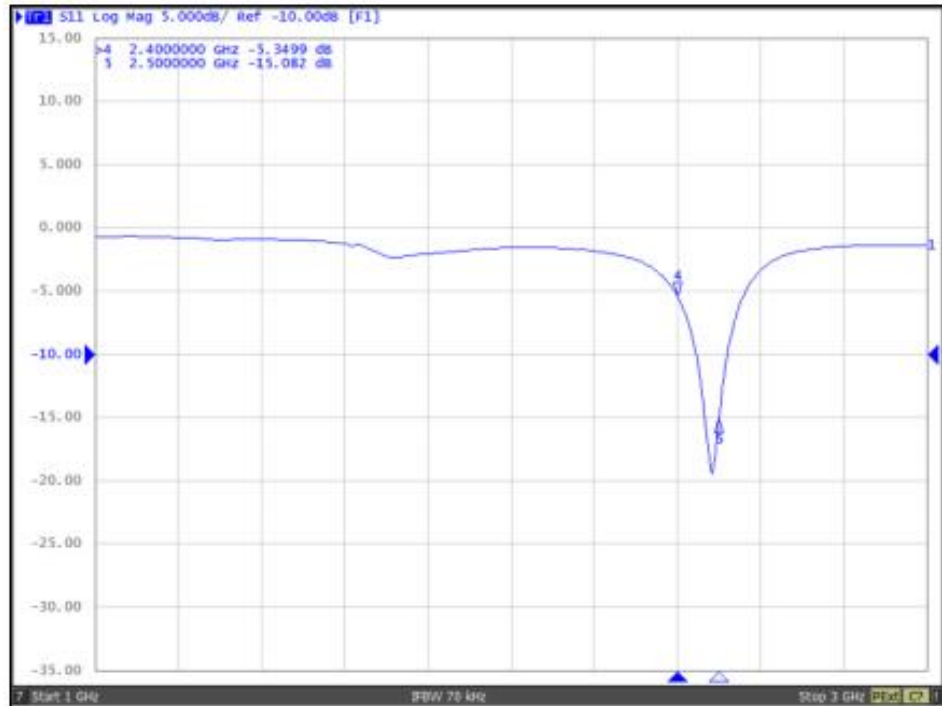
Return loss
