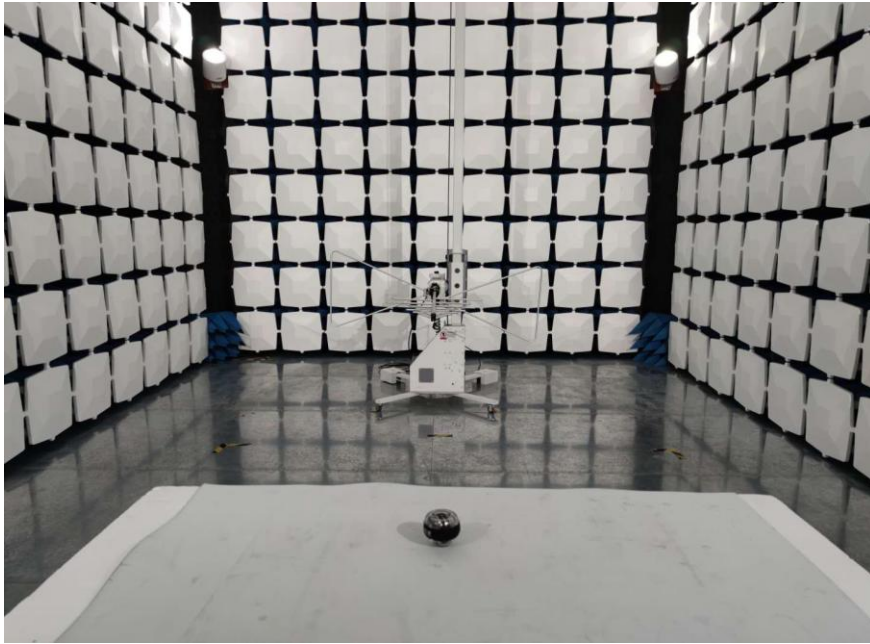
Blow 1GHz for radiated emission test setup
