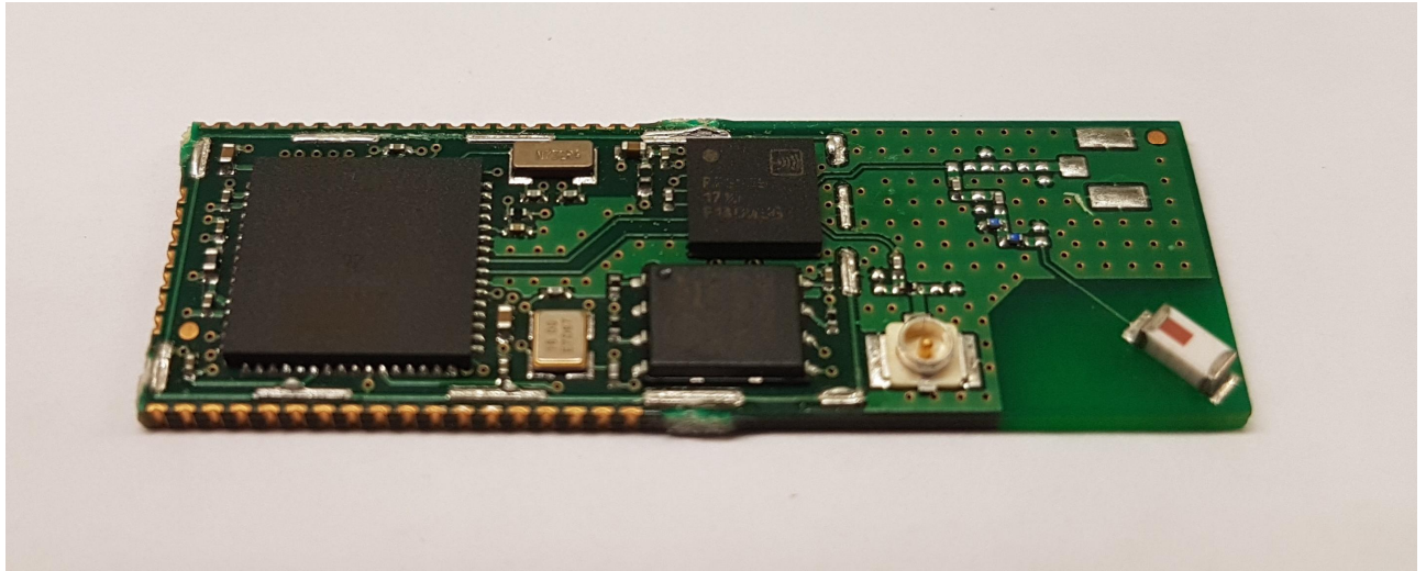
EUT Unshielded Module (AT-ANY-2400-SC3-1)*
