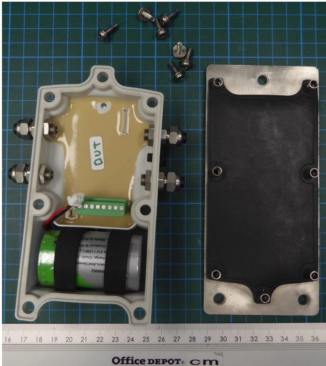
EUT Opened view
