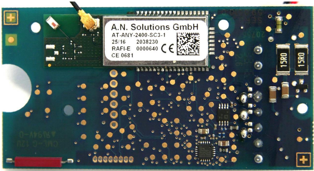
EUT Inside view – PCB bottom view*
