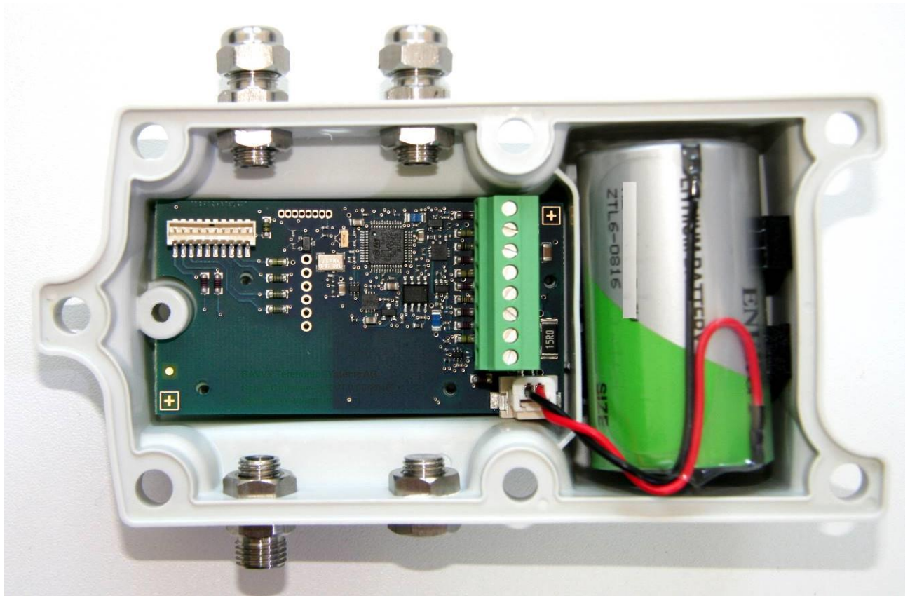
EUT Inside view – PCB top view*
