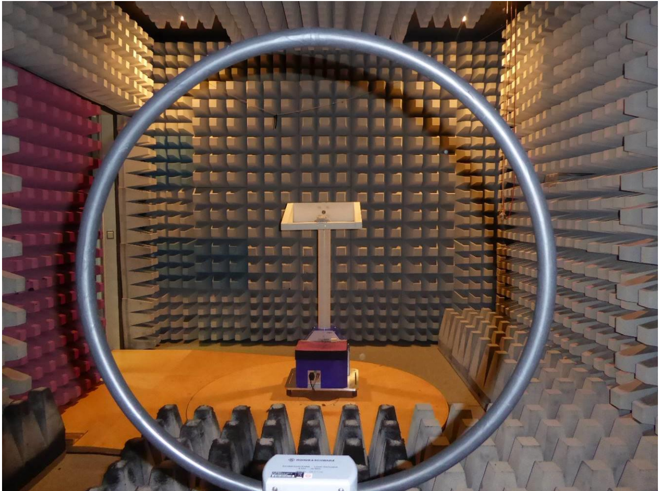
Test setup – radiated test in anechoic chamber Preliminary measurement 9 kHz - 30 MHz
