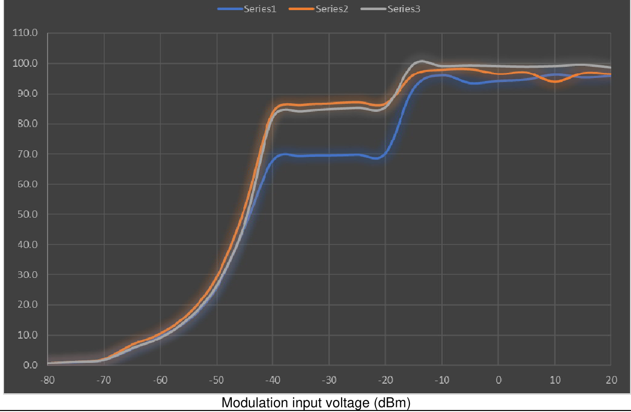
Percentage of modulation - 25 kHz Channel Spacing
