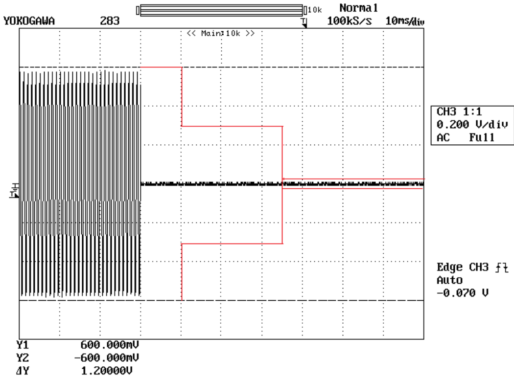
Transient Frequency behavior with modulation FM 12.5 kHz at 450.1 MHz, switch ON
