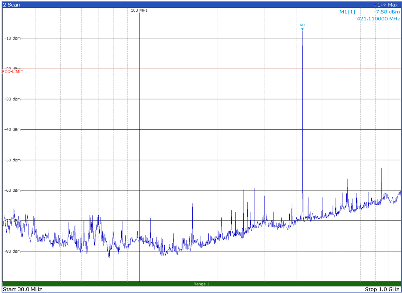
Radiated spurious emissions with modulation CST 4FSK at 421.1 MHz – Antenna in vertical polarization
