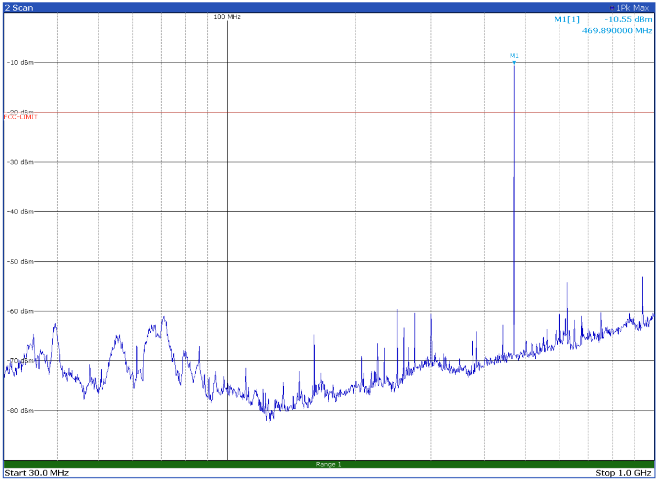
Radiated spurious emissions with modulation P25 C4FM at 469.9 MHz – Antenna in vertical polarization
