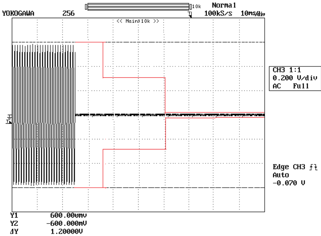
Transient Frequency behavior with modulation FM 12.5 kHz at 421.1 MHz, switch ON
