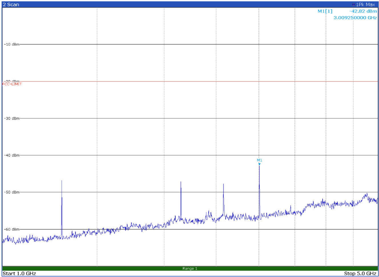
Radiated spurious emissions with modulation CST 4FSK at 429.9 MHz – Antenna in vertical polarization
