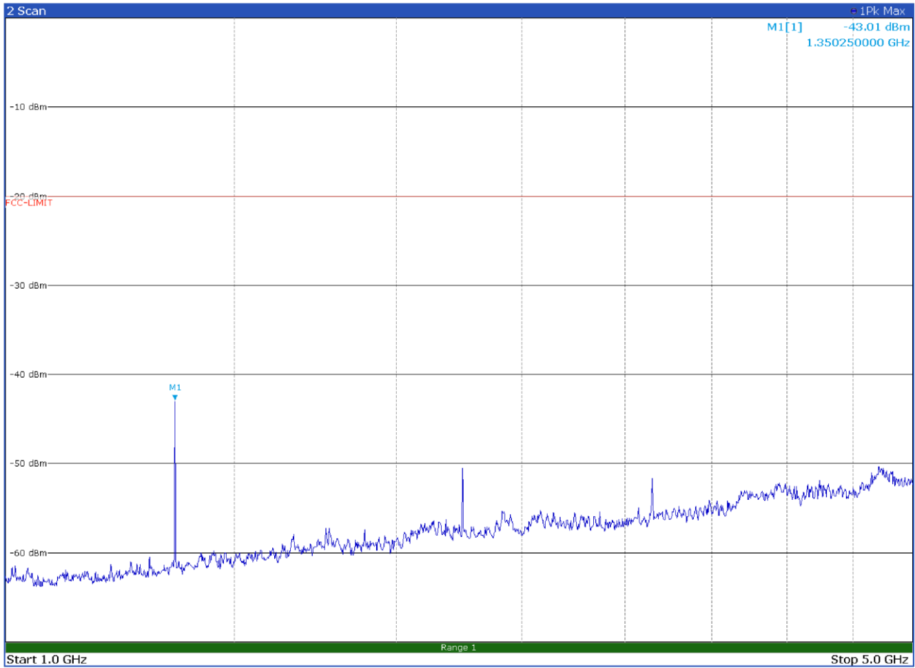
Radiated spurious emissions with modulation P25 C4FM at 450.1 MHz – Antenna in horizontal polarization
