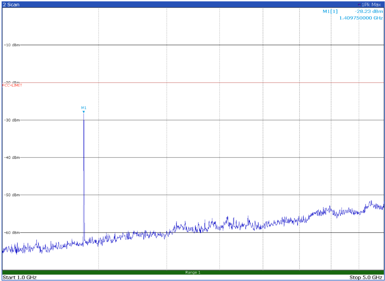
Radiated spurious emissions with modulation CST 4FSK at 469.9 MHz – Antenna in vertical polarization
