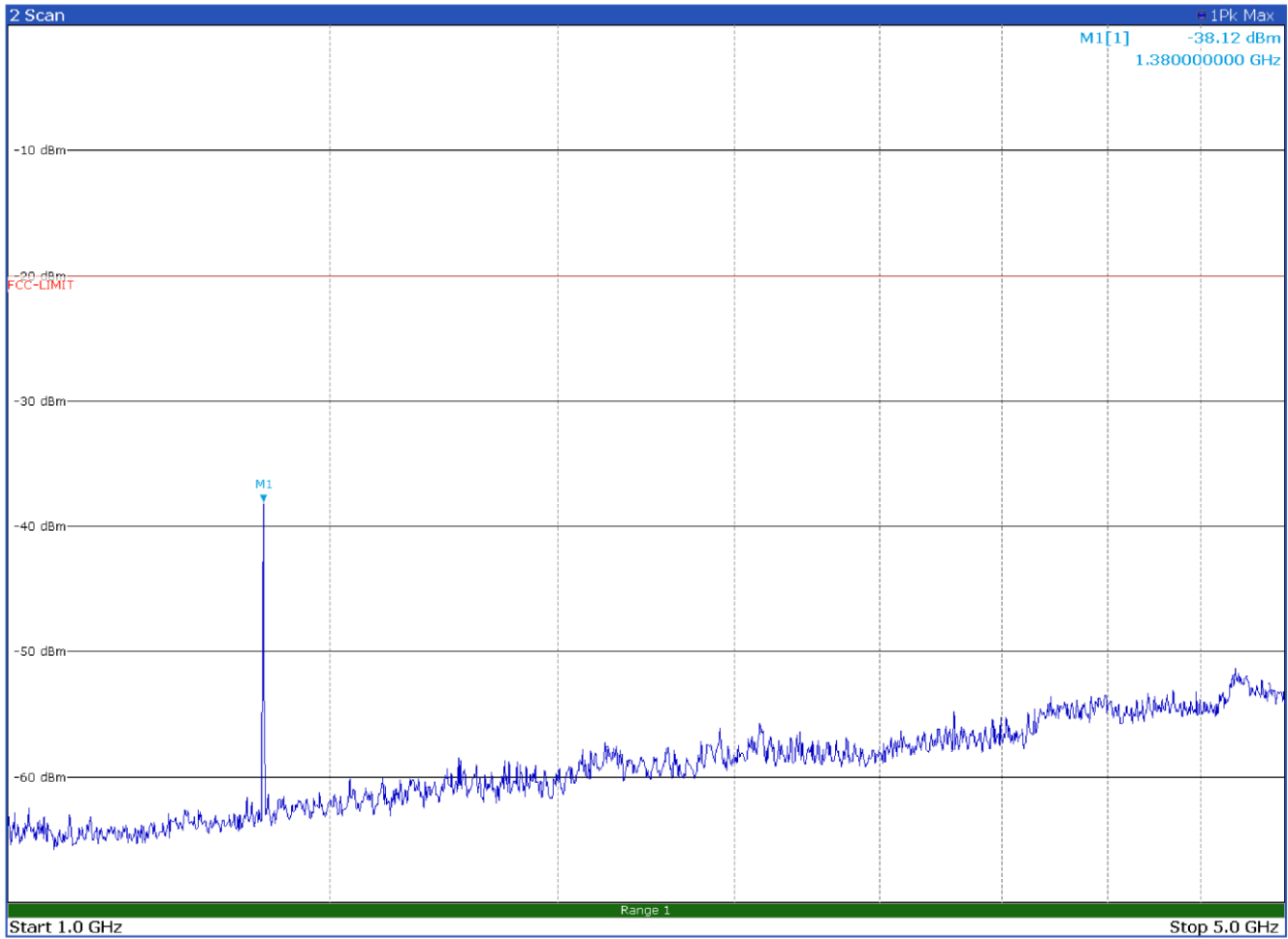
Radiated spurious emissions with modulation P25 C4FM at 460.0 MHz – Antenna in horizontal polarization
