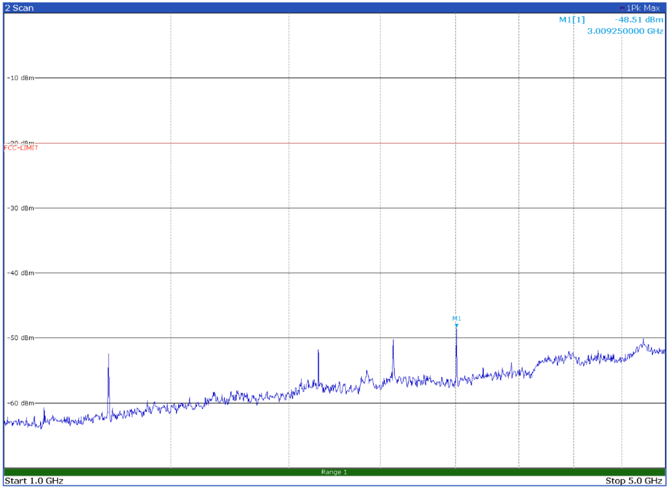
Radiated spurious emissions with modulation P25 C4FM at 429.9 MHz – Antenna in horizontal polarization
