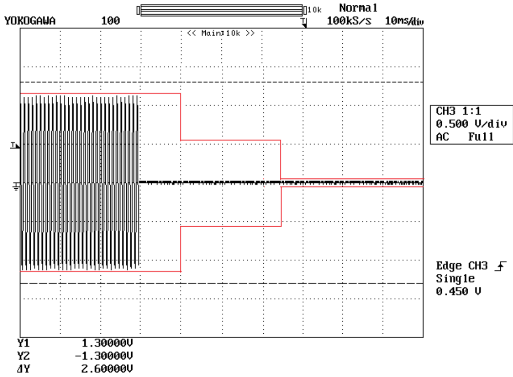
Transient Frequency behavior with modulation FM 25 kHz at 450.1 MHz, switch ON
