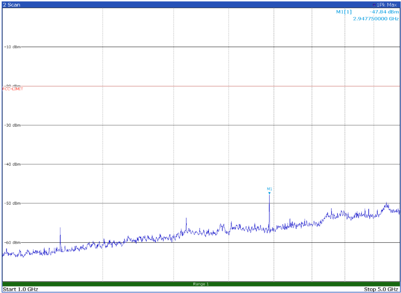
Radiated spurious emissions with modulation CST 4FSK at 421.1 MHz – Antenna in horizontal polarization
