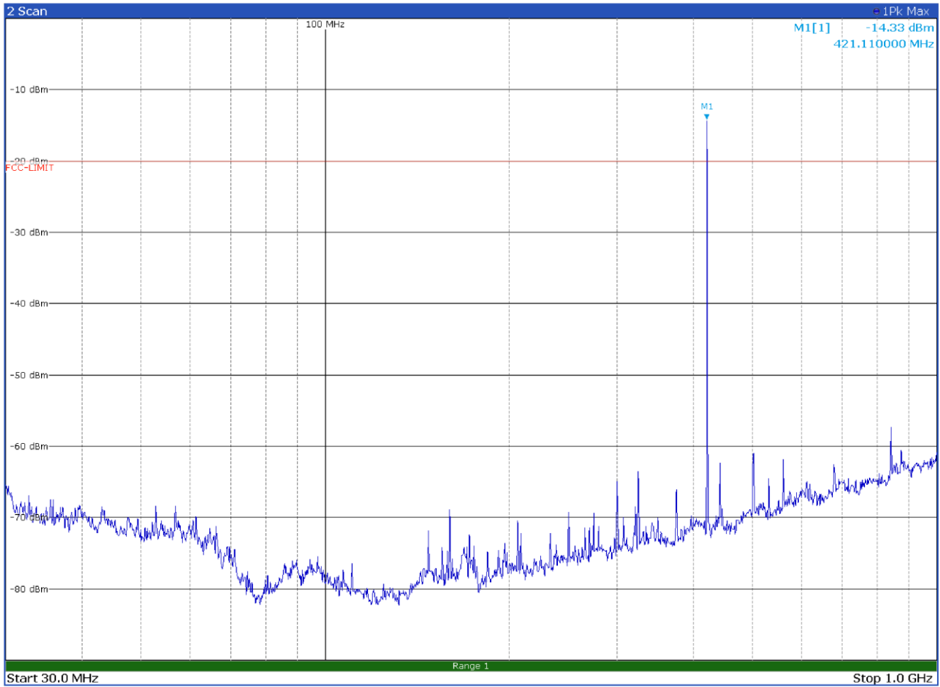
Radiated spurious emissions with modulation P25 C4FM at 421.1 MHz – Antenna in horizontal polarization
