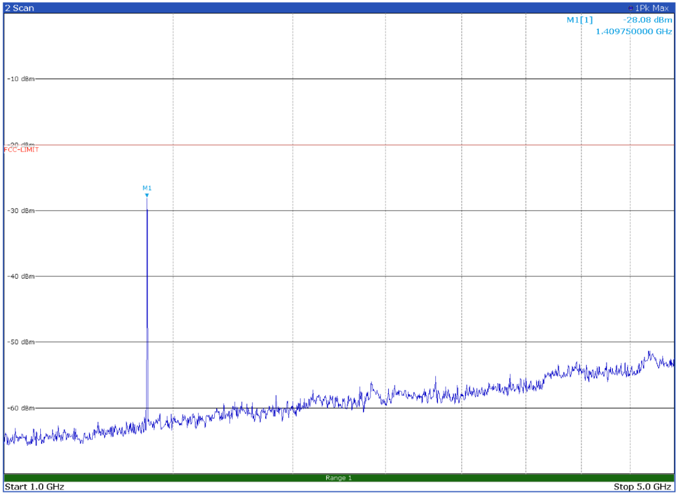
Radiated spurious emissions with modulation FM 25.0 kHz at 469.9 MHz – Antenna in vertical polarization
