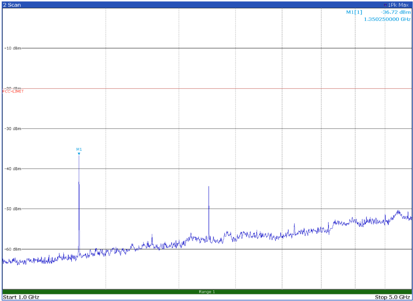
Radiated spurious emissions with modulation P25 C4FM at 450.1 MHz – Antenna in vertical polarization
