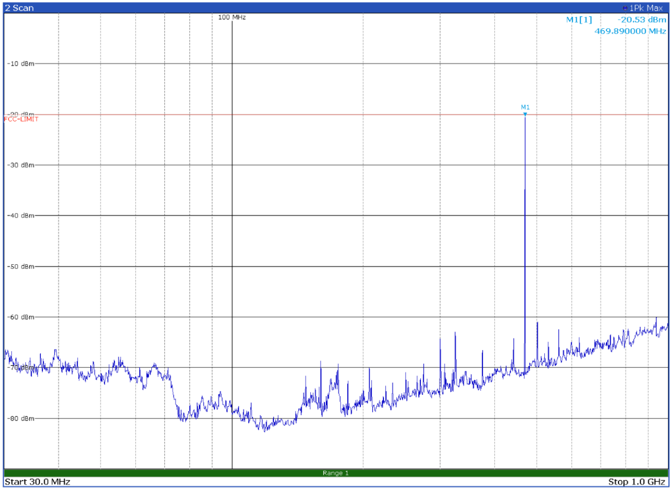
Radiated spurious emissions with modulation CST 4FSK at 469.9 MHz – Antenna in horizontal polarization
