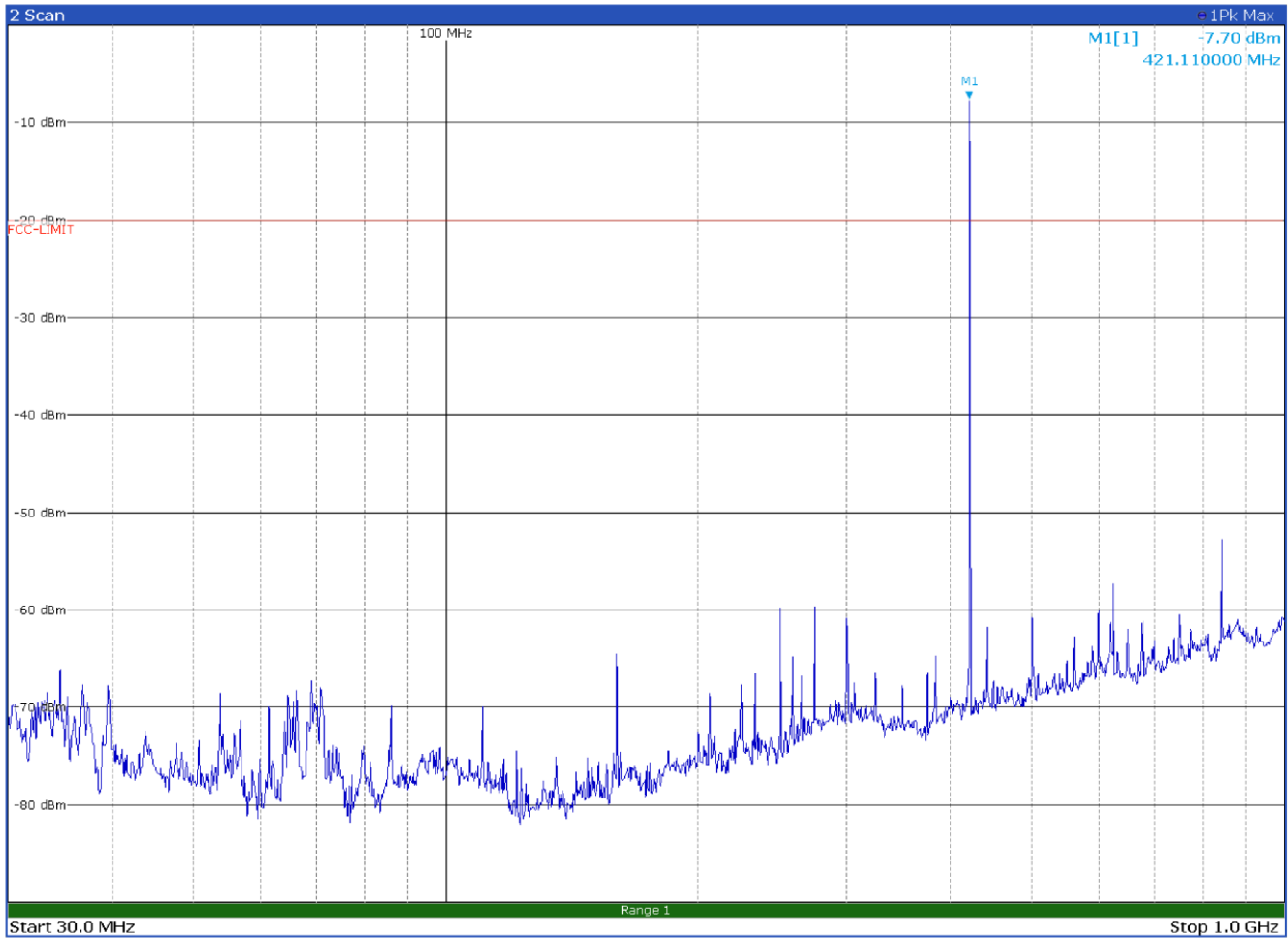
Radiated spurious emissions with modulation P25 C4FM at 421.1 MHz – Antenna in vertical polarization
