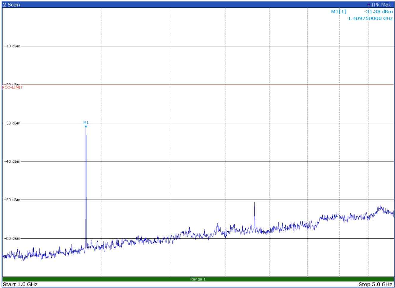
Radiated spurious emissions with modulation FM 25.0 kHz at 469.9 MHz – Antenna in horizontal polarization
