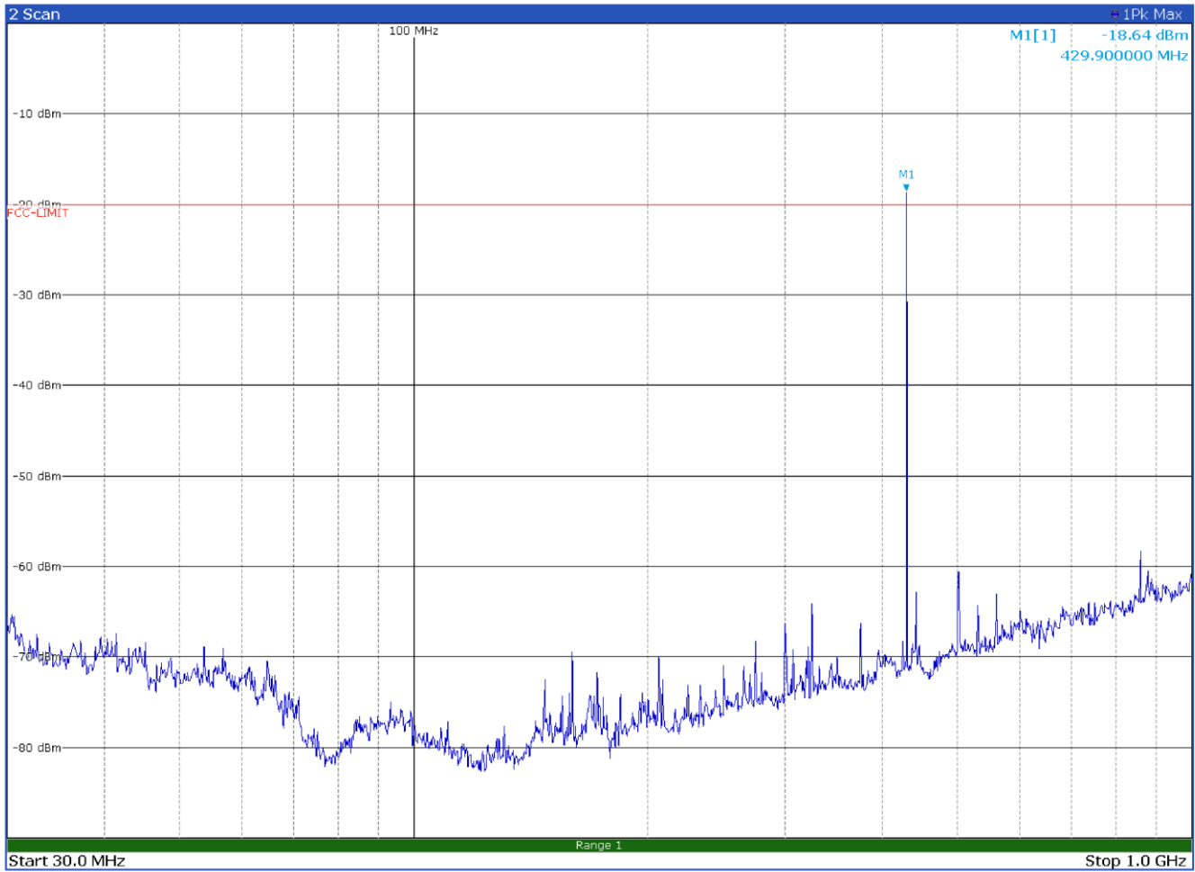
Radiated spurious emissions with modulation CST 4FSK at 429.9 MHz – Antenna in horizontal polarization
