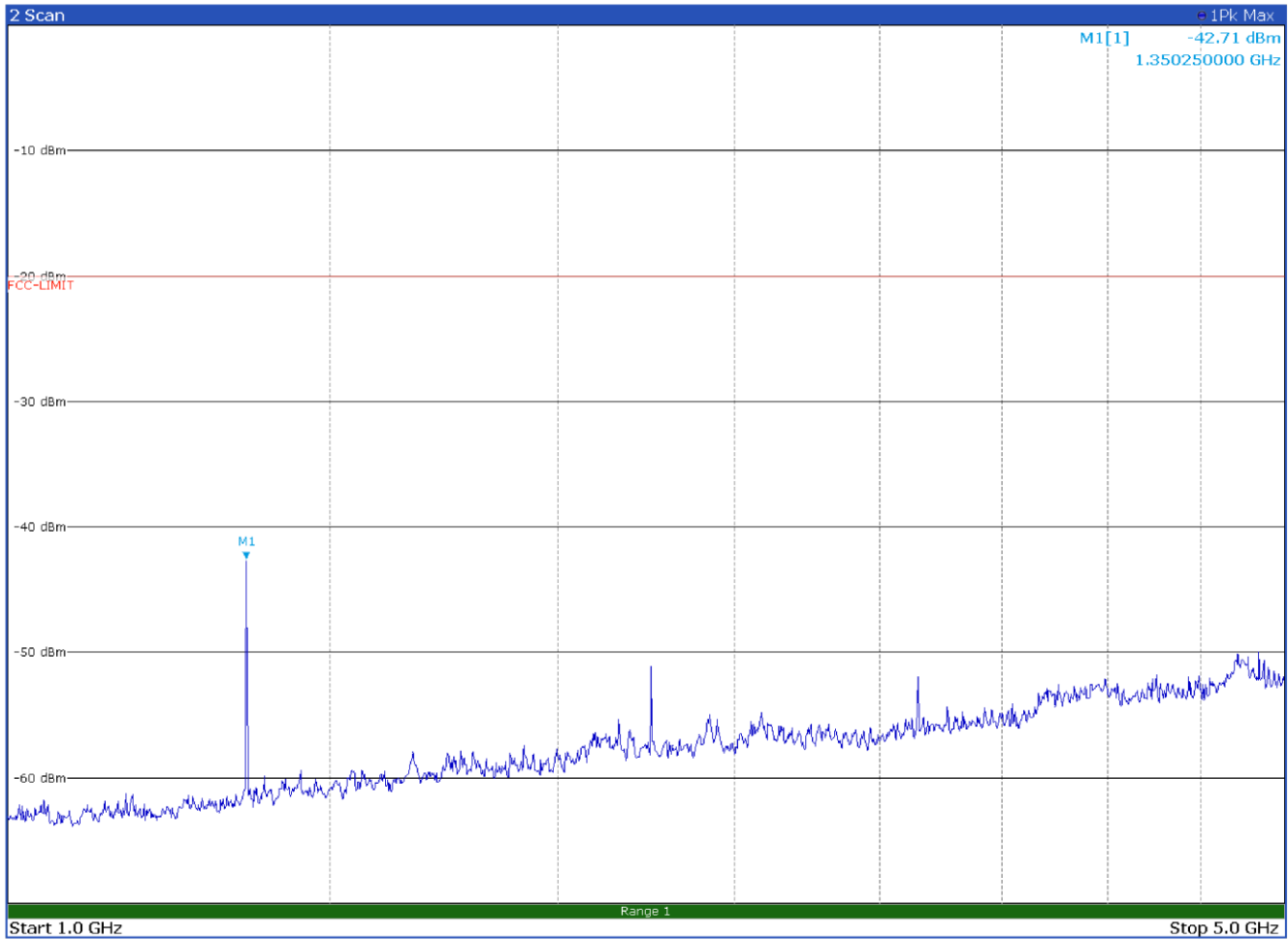
Radiated spurious emissions with modulation CST 4FSK at 450.1 MHz – Antenna in horizontal polarization
