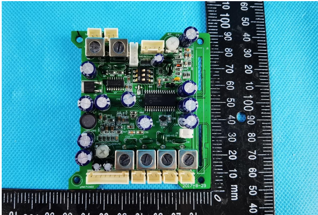
Master controller
