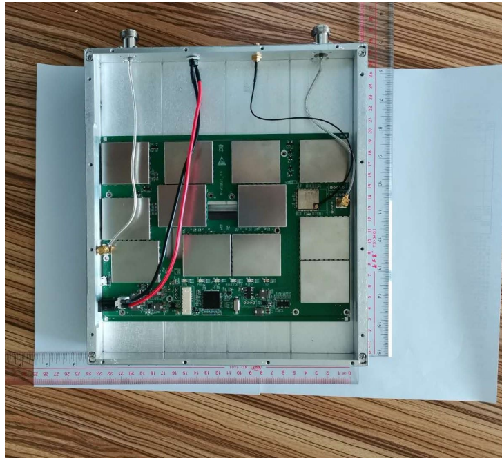
EUT – PCB Top View
