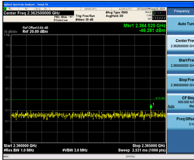
Band40-5MHz-16QAM-39175-1RB#0-Range6:2365~26500MHz
