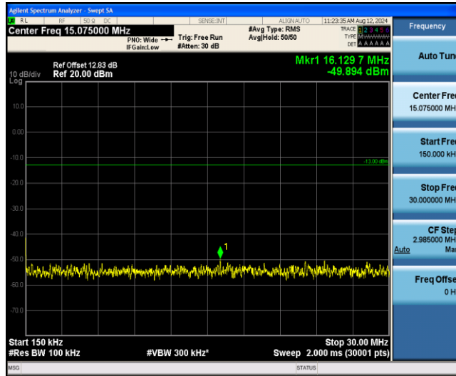
Band26-3MHz-16QAM-26775-1RB#0-Range3:30~1000MHz
