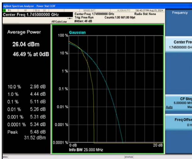
Band66-10MHz-16QAM-132322-27RB#0
