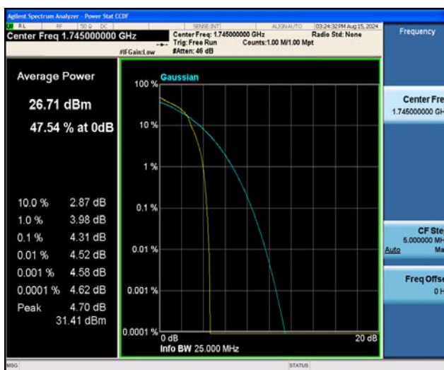
Band66-5MHz-16QAM-132322-25RB#0
