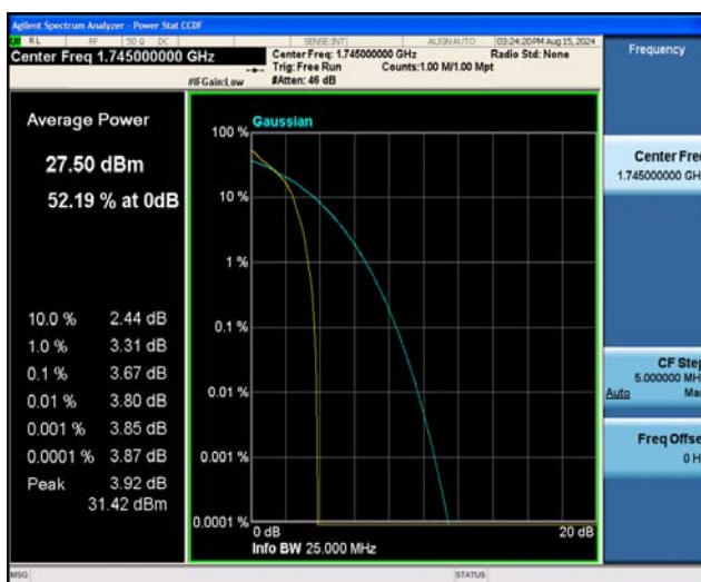
Band66-5MHz-QPSK-132322-25RB#0
