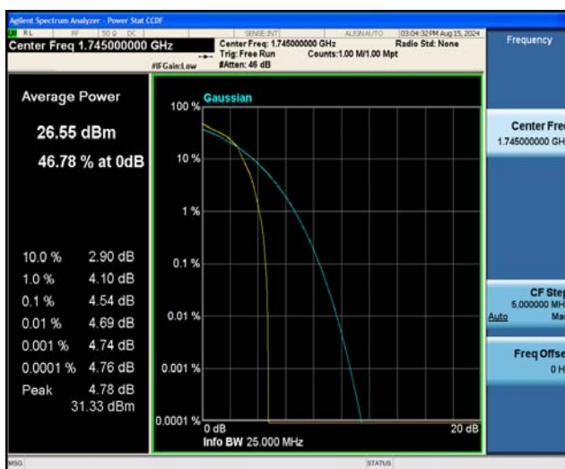
Band66-3MHz-16QAM-132322-15RB#0
