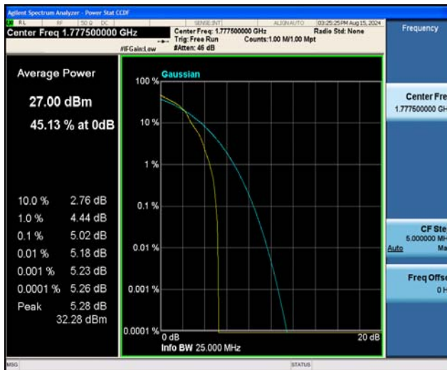
Band66-5MHz-16QAM-132647-25RB#0
