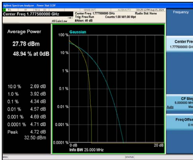
Band66-5MHz-QPSK-132647-25RB#0
