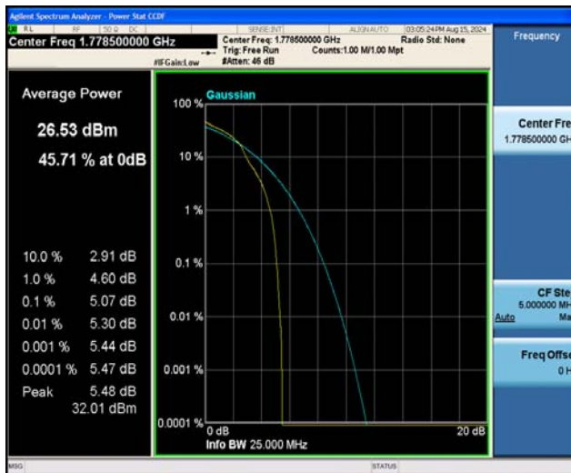
Band66-3MHz-16QAM-132657-15RB#0
