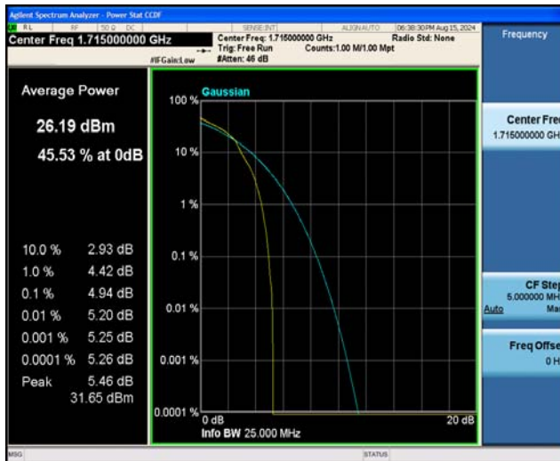
Band66-10MHz-16QAM-132022-27RB#0
