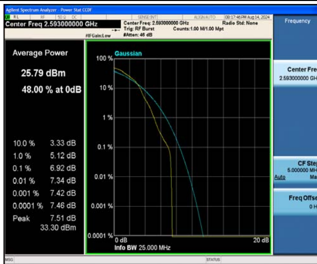
Band41-10MHz-16QAM-40620-27RB#0
