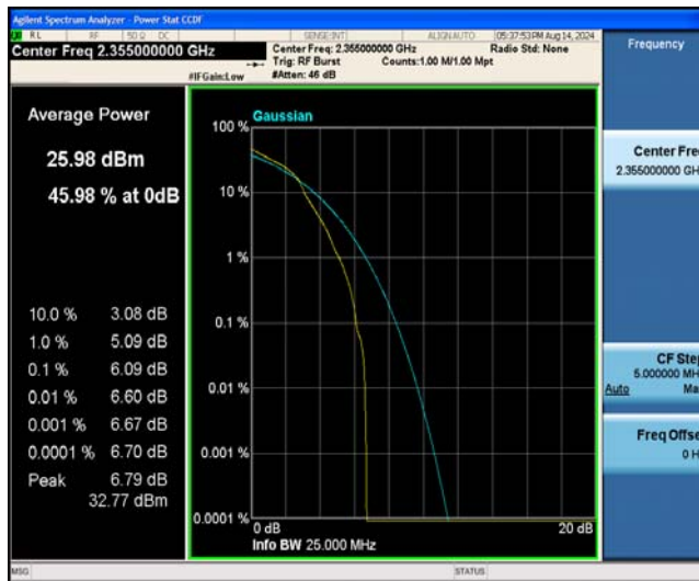
Band40-10MHz-16QAM-39200-27RB#0
