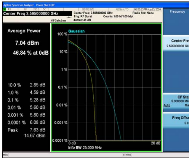
Band38-20MHz-16QAM-38000-27RB#0
