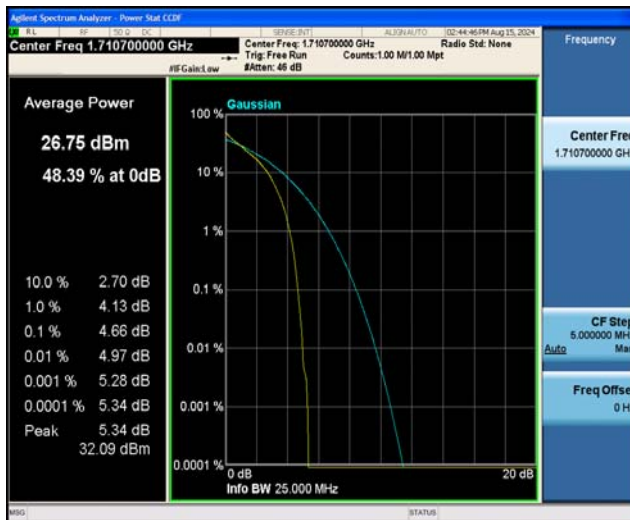
Band66-1.4MHz-QPSK-132322-1RB#0
