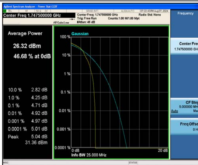
Band4-15MHz-16QAM-20325-27RB#0
