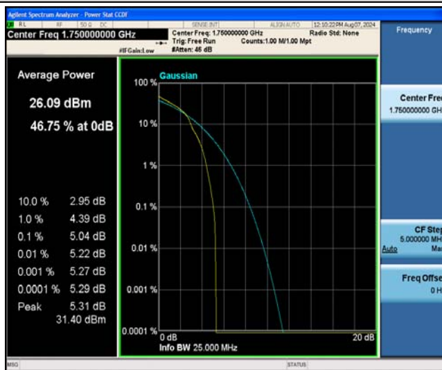
Band4-10MHz-16QAM-20350-27RB#0
