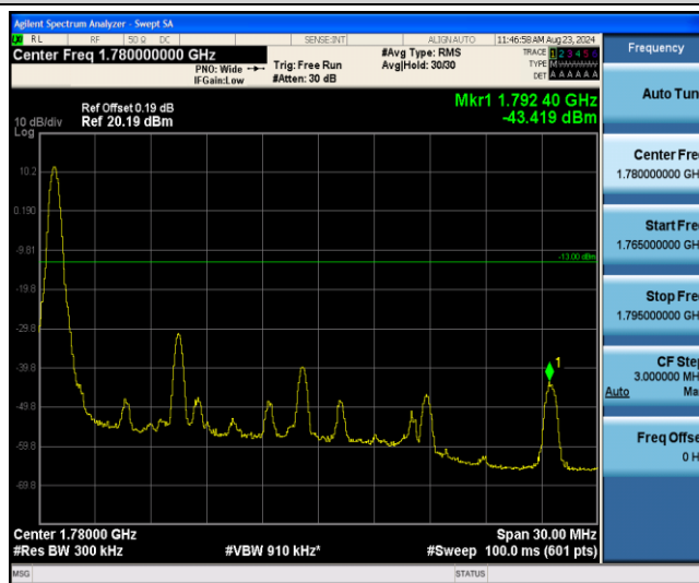
Band66-15MHz-16QAM-132597-27RB#0
