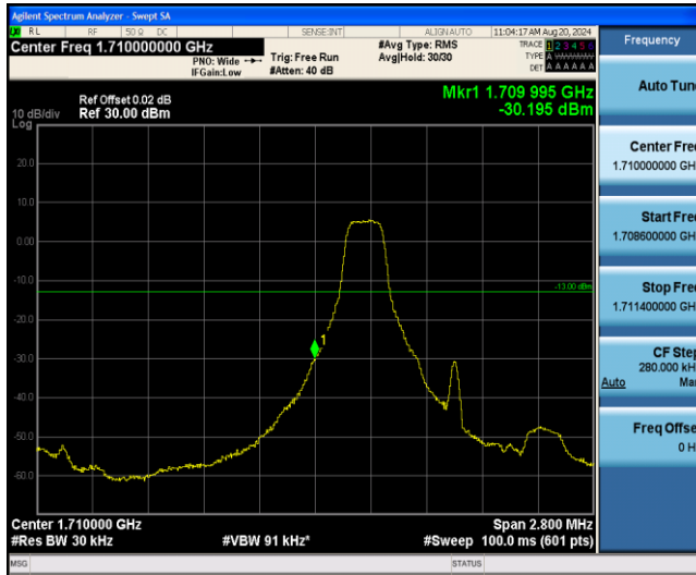
Band66-1.4MHz-QPSK-131979-1RB#5
