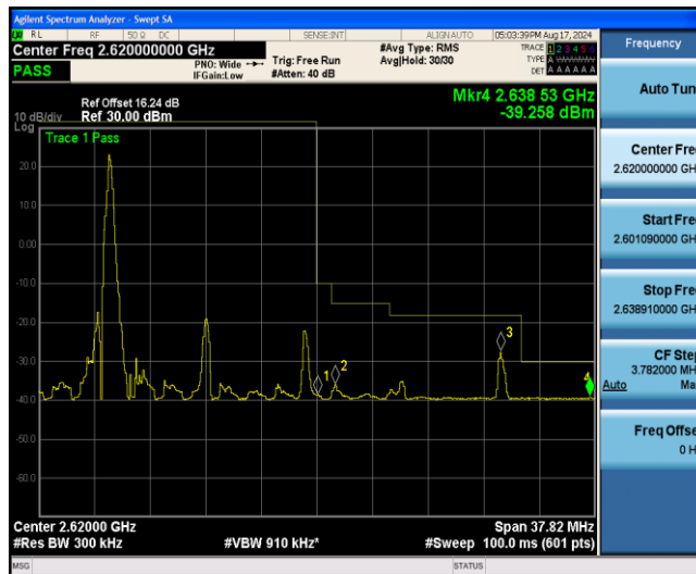
Band38-15MHz-16QAM-38175-27RB#0
