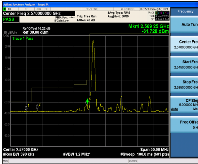
Band38-20MHz-16QAM-37850-27RB#0
