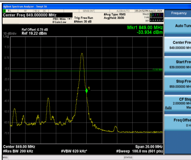
Band26-10MHz-16QAM-26990-27RB#0
