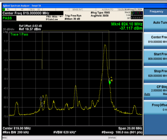
Band26-10MHz-16QAM-26740-27RB#0
