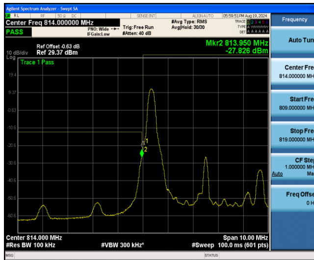
Band26-5MHz-QPSK-26715-1RB#24
