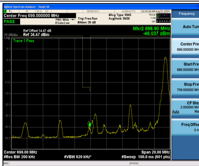
Band12-10MHz-16QAM-23060-27RB#0
