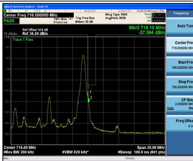
Band12-10MHz-16QAM-23130-27RB#0
