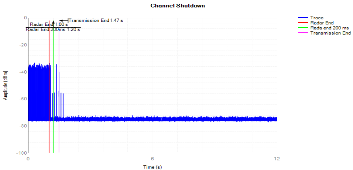
5530MHz ac80 Shutdown
