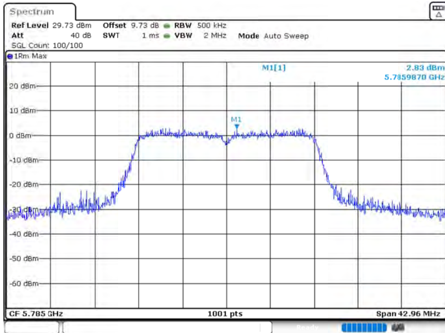
PSD NVNT 802.11ac20 5785MHz Ant1
