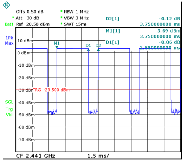
Middle Channel
