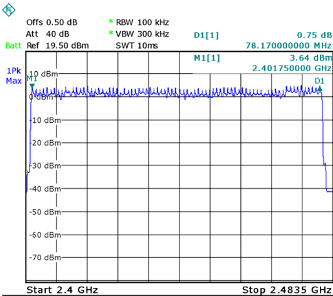
Modulation: 8DPSK
