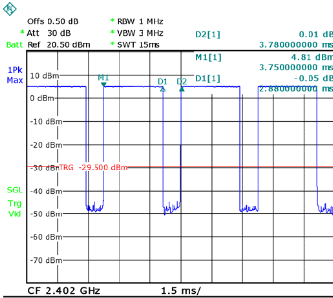
Low Channel
