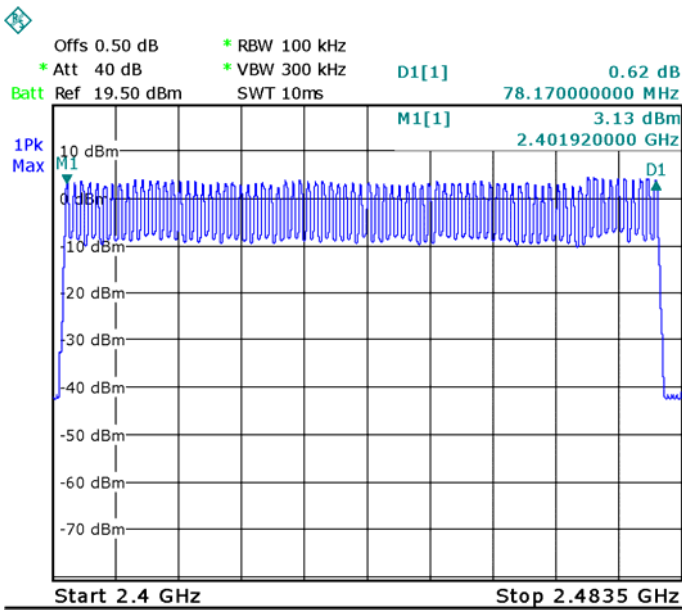
Modulation: 8DPSK
