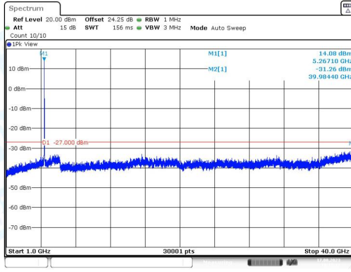
11N20SISO_Ant1_5260_1000~40000
