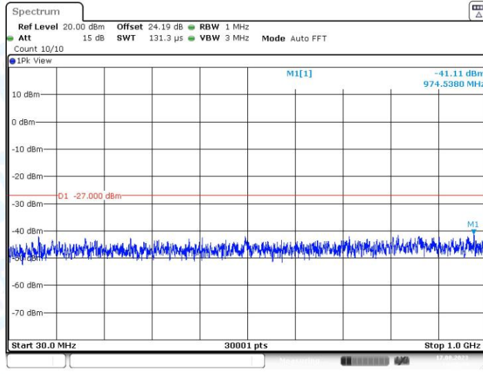
11N40SISO_Ant1_5270_30~1000
