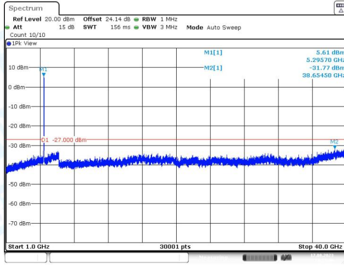
11N40SISO_Ant1_5310_1000~40000
