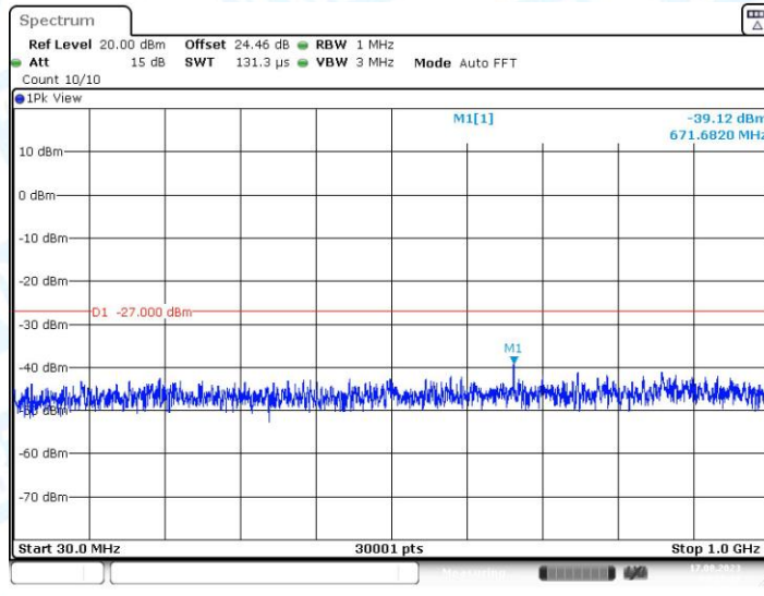
11A_Ant1_5825_30~1000
