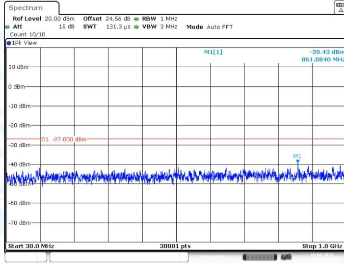
11A_Ant1_5500_30~1000
