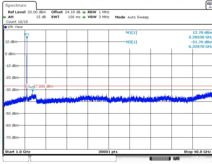
11N20SISO_Ant1_5280_1000~40000
