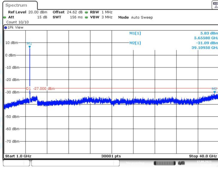
11N40SISO_Ant1_5670_1000~40000
