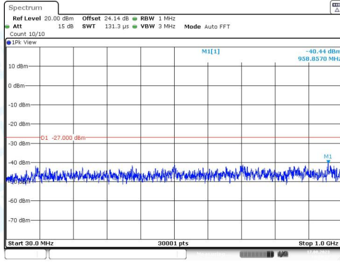
11N40SISO_Ant1_5310_30~1000
