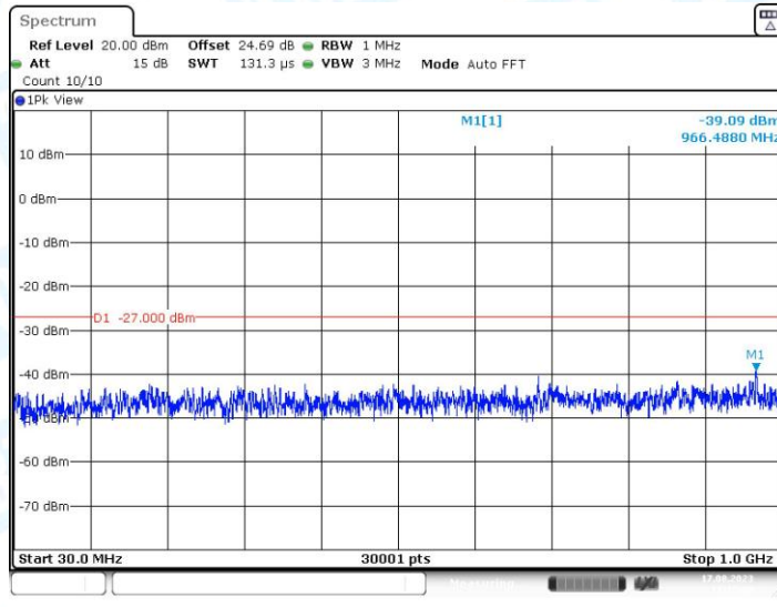
11N20SISO_Ant1_5700_30~1000
