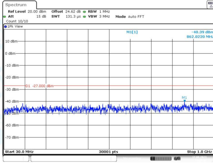
11N40SISO_Ant1_5670_30~1000
