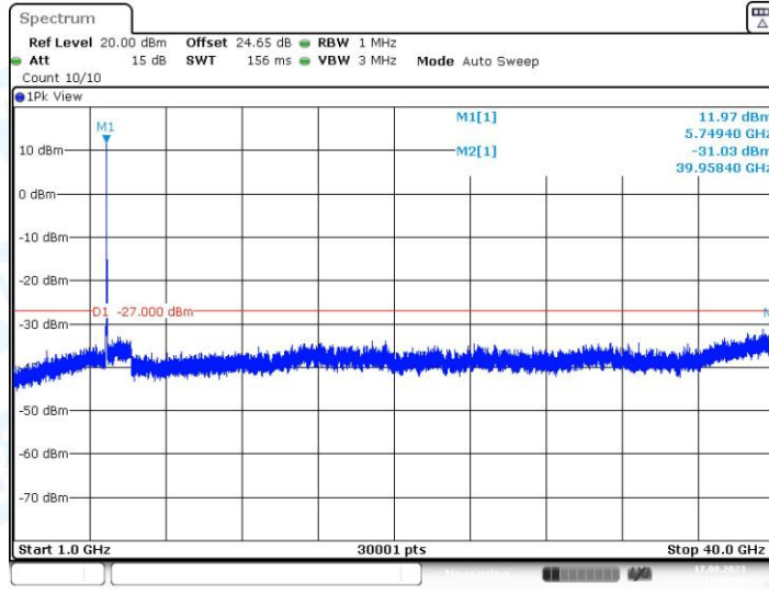
11N20SISO_Ant1_5745_1000~40000
