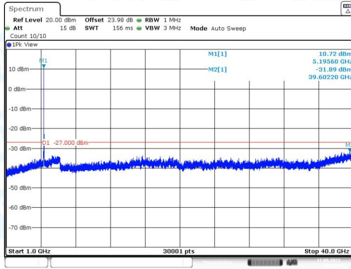
11AC20SISO_Ant1_5200_1000~40000
