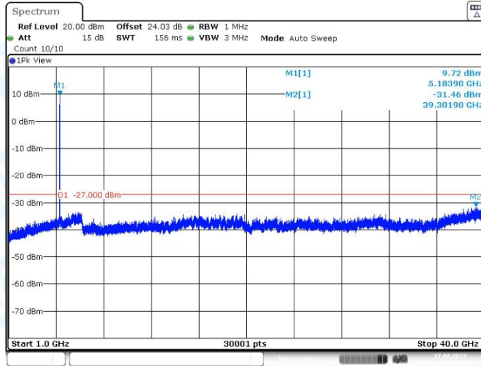
11AC20SISO_Ant1_5180_1000~40000
