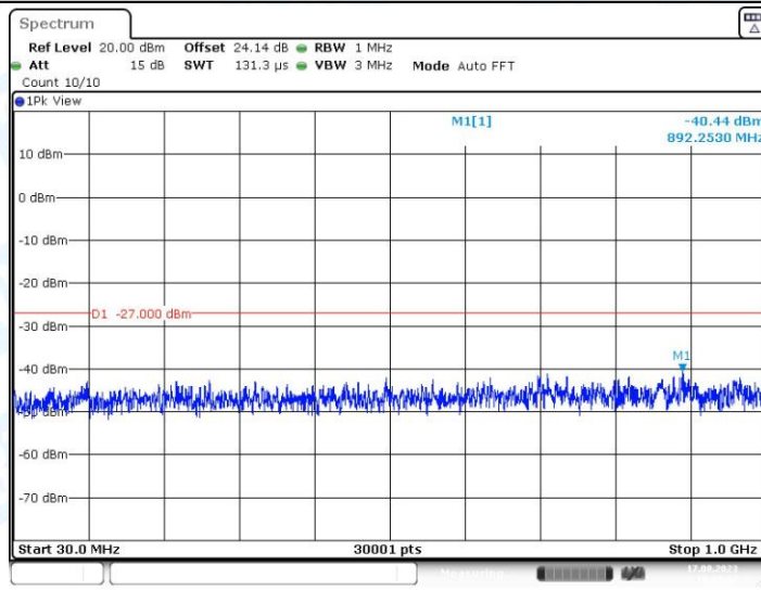
11N20SISO_Ant1_5320_30~1000
