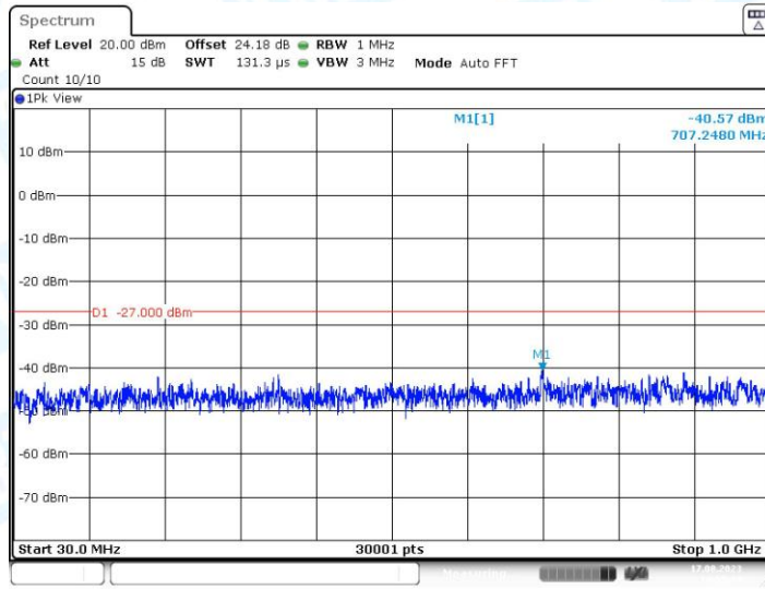
11AC20SISO_Ant1_5240_30~1000
