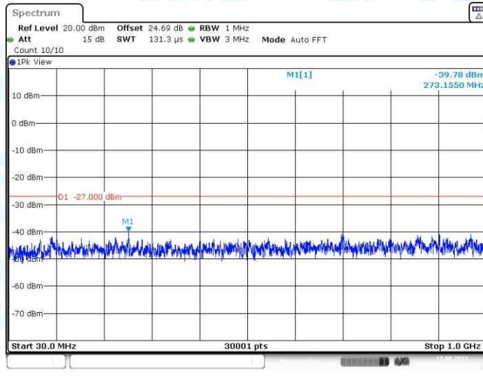
11A_Ant1_5700_30~1000
