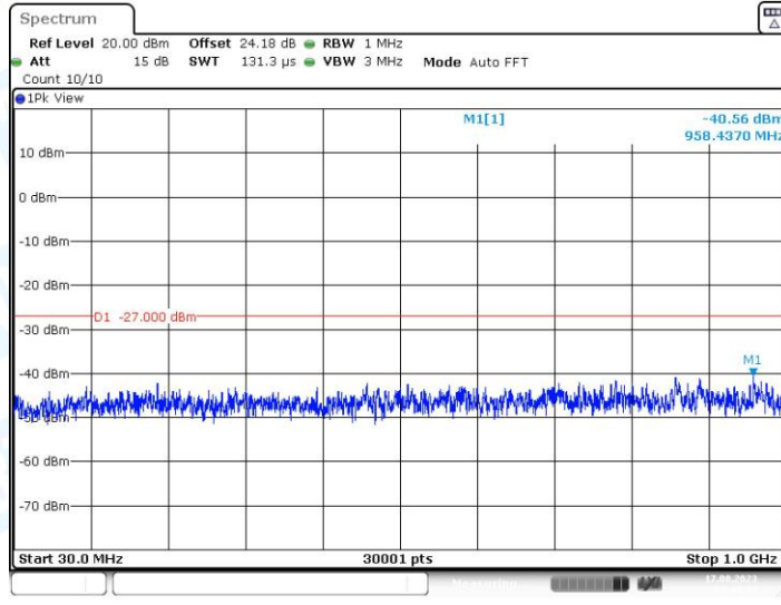
11N20SISO_Ant1_5240_30~1000
