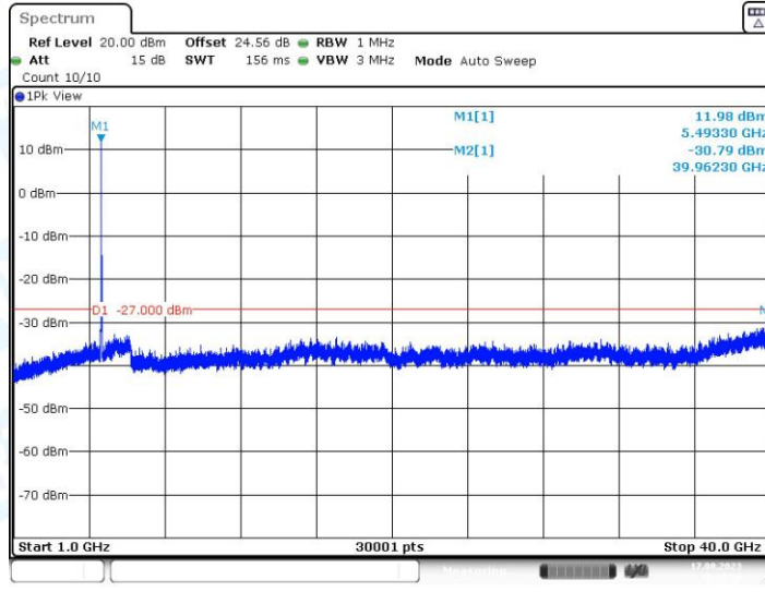
11N20SISO_Ant1_5500_1000~40000
