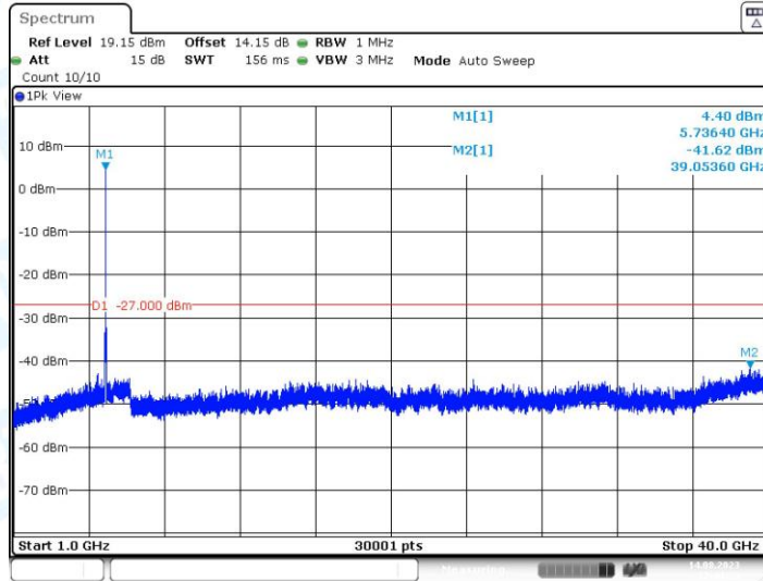
11AC20MIMO_Ant1_5745_1000~40000
