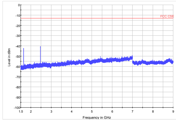
NB-IOT Band 26 CH-Middle 1.5GHz~9GHz
