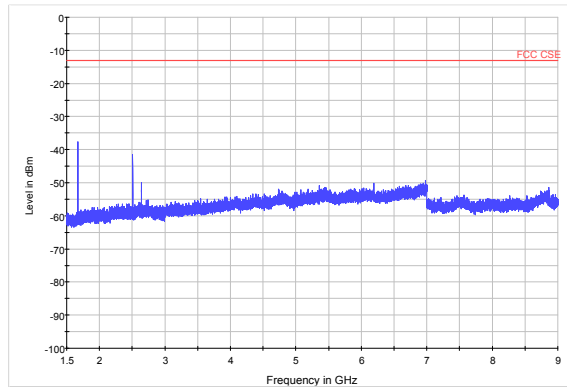
NB-IOT Band 26 CH-High 1.5GHz~9GHz
