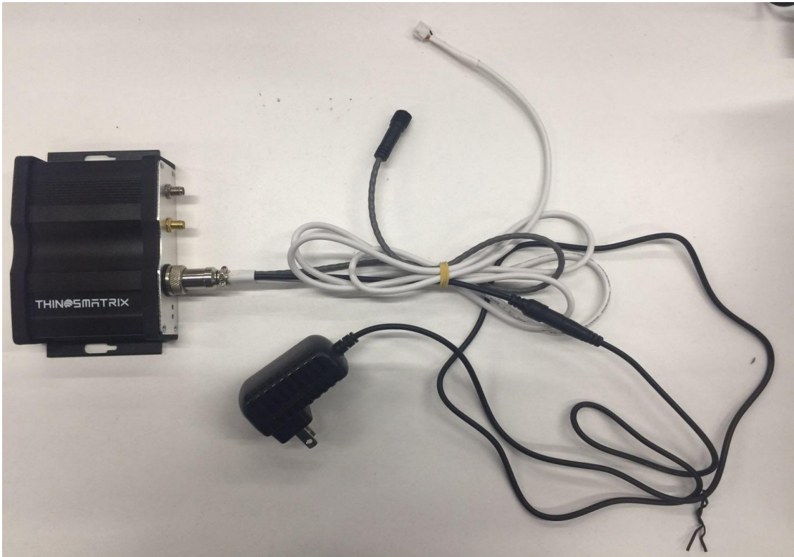
3) Connection the Current Draw Sensor to the main cable
