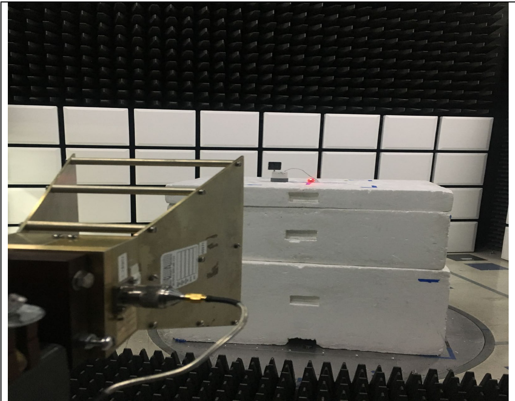
RF Radiated 1-18 GHz
