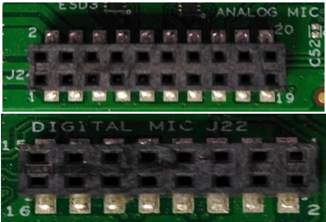
Figure 20 – IO Card Analog and Digital Codec Headers (J24 & J22)
