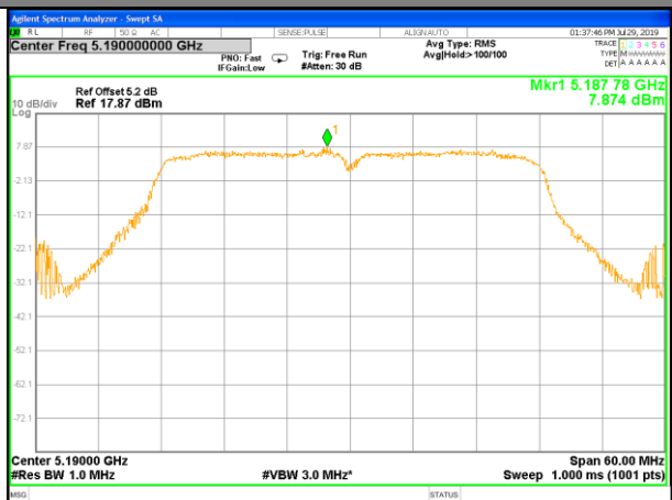
W52_11ac40_Lower_Power Spectrum Density
