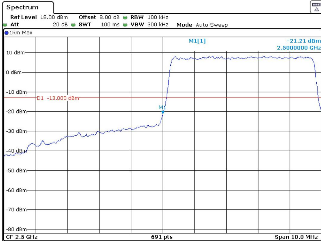
Band 7_5 MHz_Low_QPSK_RB25#0
