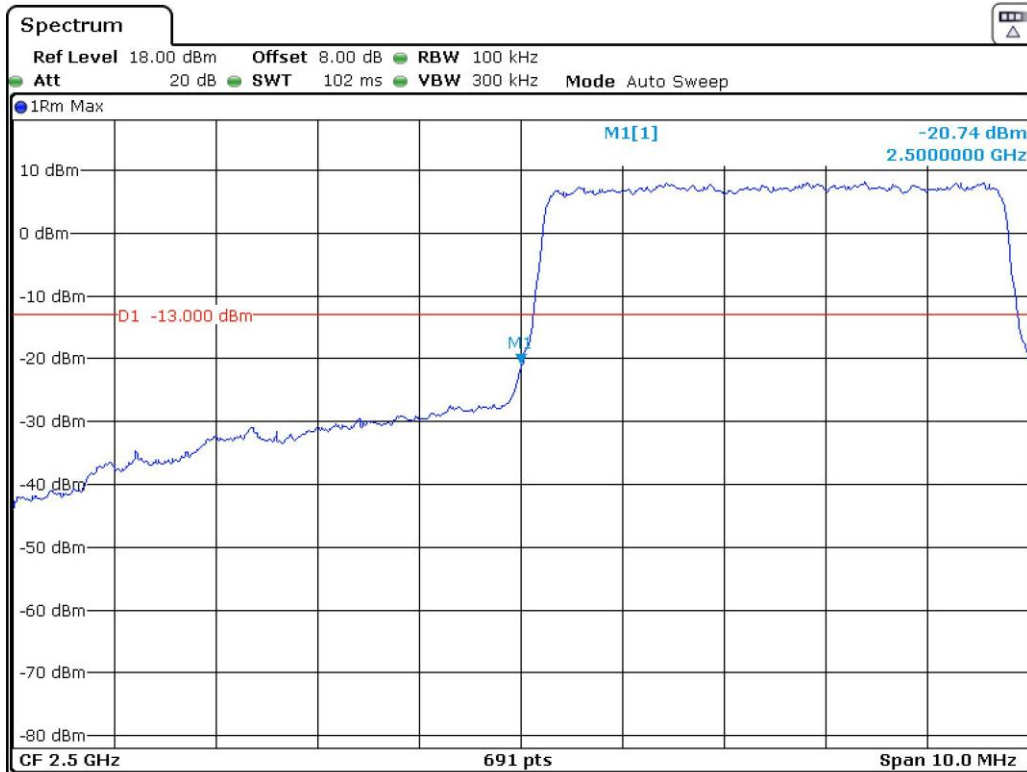
Band 7_5 MHz_Low_16QAM_RB25#0
