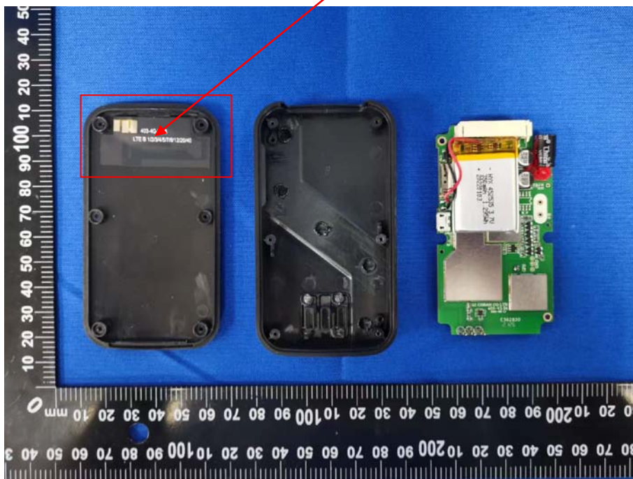
2G/4G Antenna
