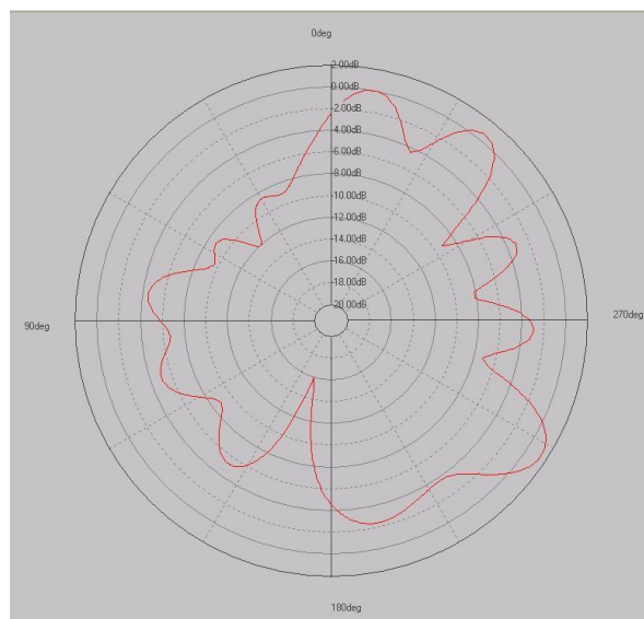
H plane
