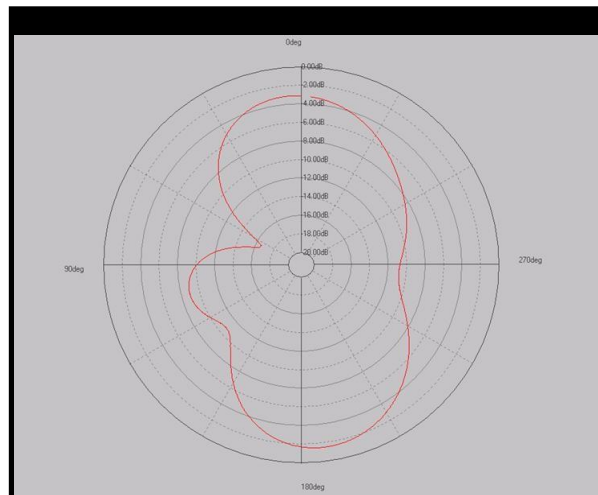
H plane
