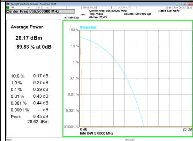
Band 5_15kHz_QPSK_Middle_1#12
