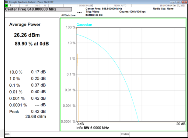
Band 5_15kHz_QPSK_High_1#12
