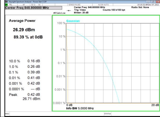
Band 5_15kHz_BPSK_High_3#0
