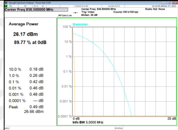
Band 5_15kHz_BPSK_Middle_3#0
