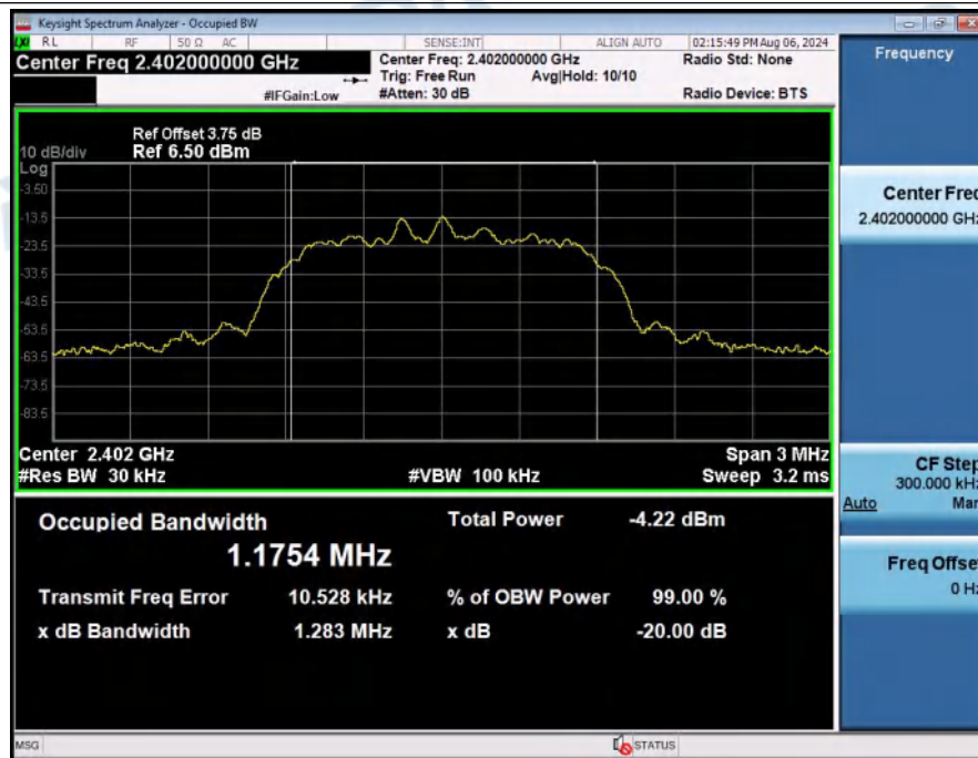
-20dB_Bandwidth_NVNT_ANT1_2-DH5_2402_00
