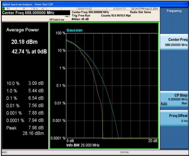
Band71-20MHz-16QAM-133372-1RB#0-PASS
