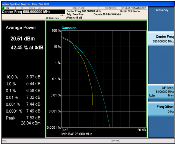
Band71-5MHz-16QAM-133297-1RB#0-PASS
