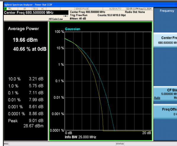
Band71-15MHz-16QAM-133297-75RB#0-PASS
