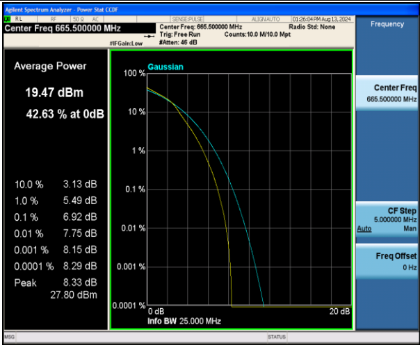
Band71-5MHz-16QAM-133147-25RB#0-PASS
