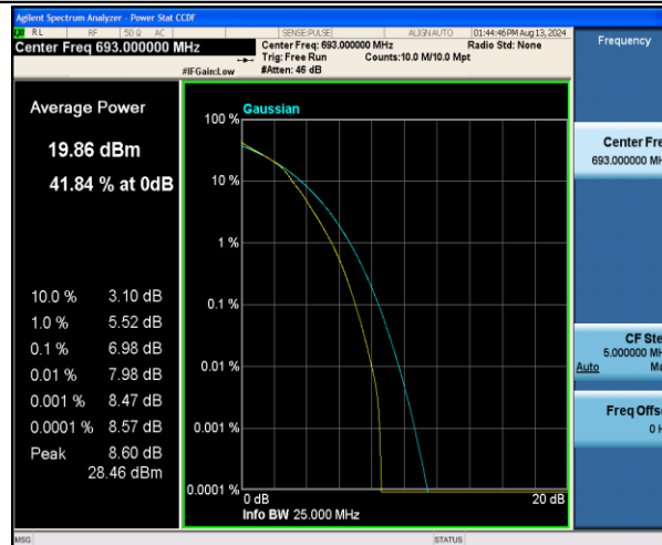
Band71-10MHz-16QAM-133422-50RB#0-PASS
