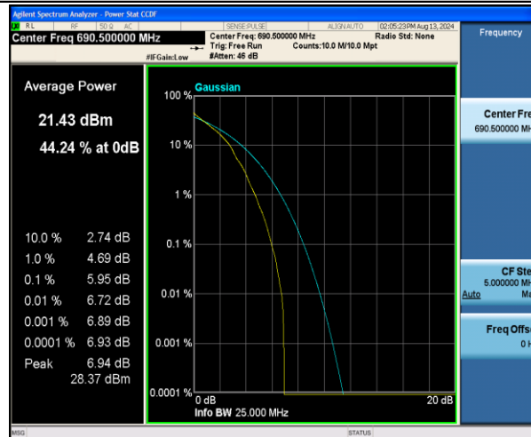
Band71-15MHz-QPSK-133397-1RB#0-PASS
