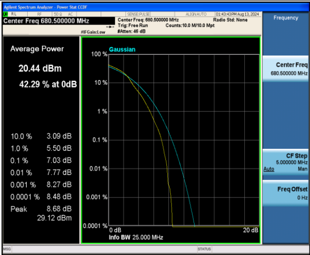
Band71-10MHz-16QAM-133297-1RB#0-PASS
