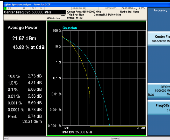
Band71-5MHz-QPSK-133447-1RB#0-PASS
