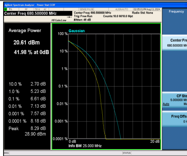
Band71-15MHz-QPSK-133297-75RB#0-PASS
