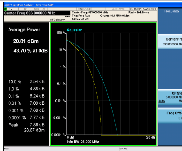
Band71-10MHz-QPSK-133422-50RB#0-PASS
