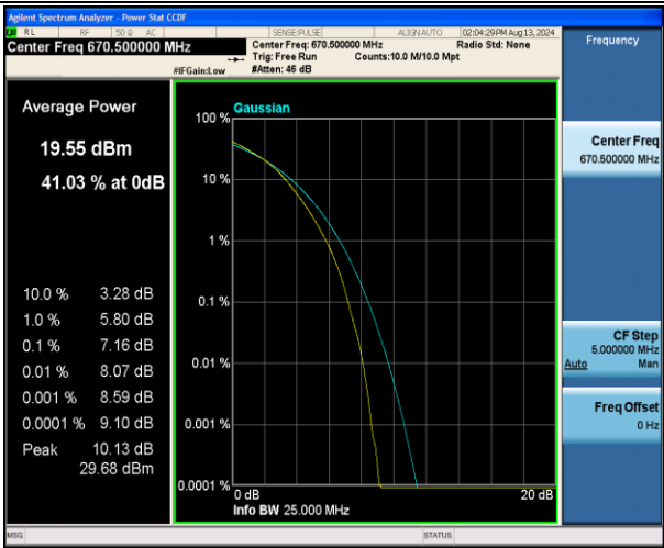
Band71-15MHz-16QAM-133197-75RB#0-PASS
