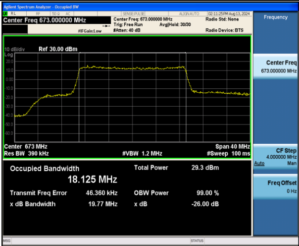
Band71-20MHz-16QAM-133222-100RB#0-PASS
