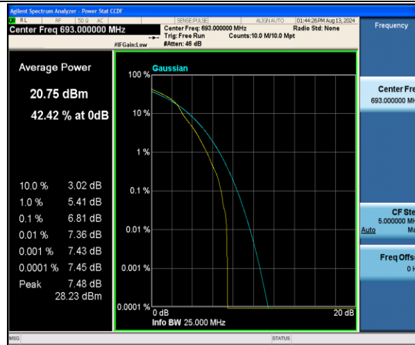
Band71-10MHz-16QAM-133422-1RB#0-PASS
