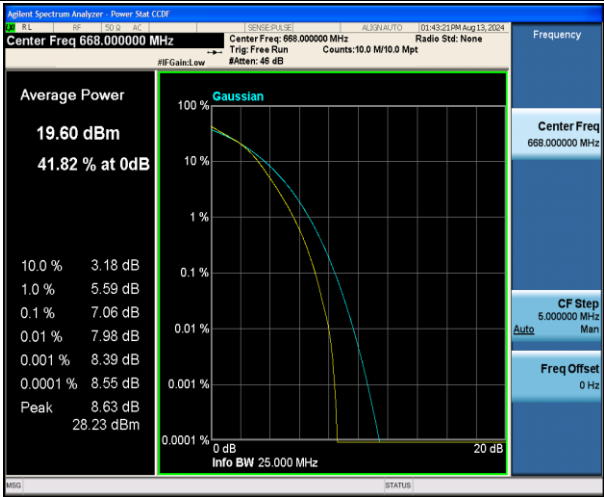
Band71-10MHz-16QAM-133172-50RB#0-PASS
