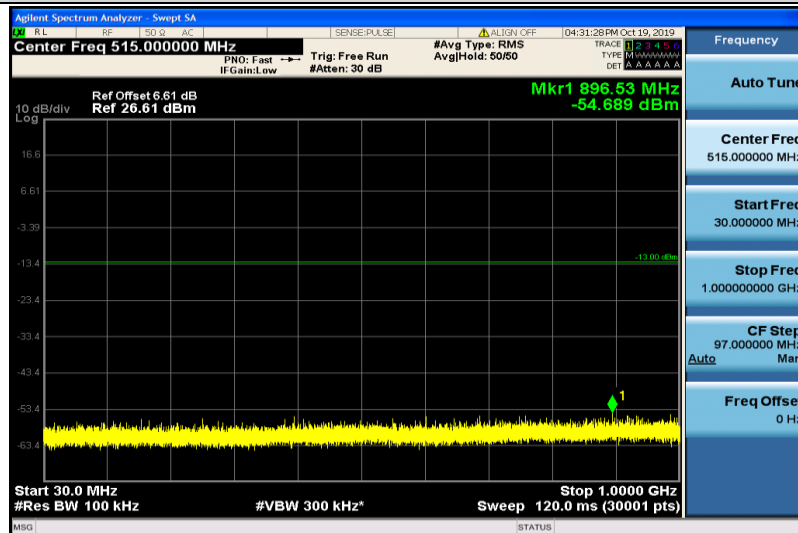
Band4-5MHz-QPSK-20175-1RB#0-30~1000MHz
