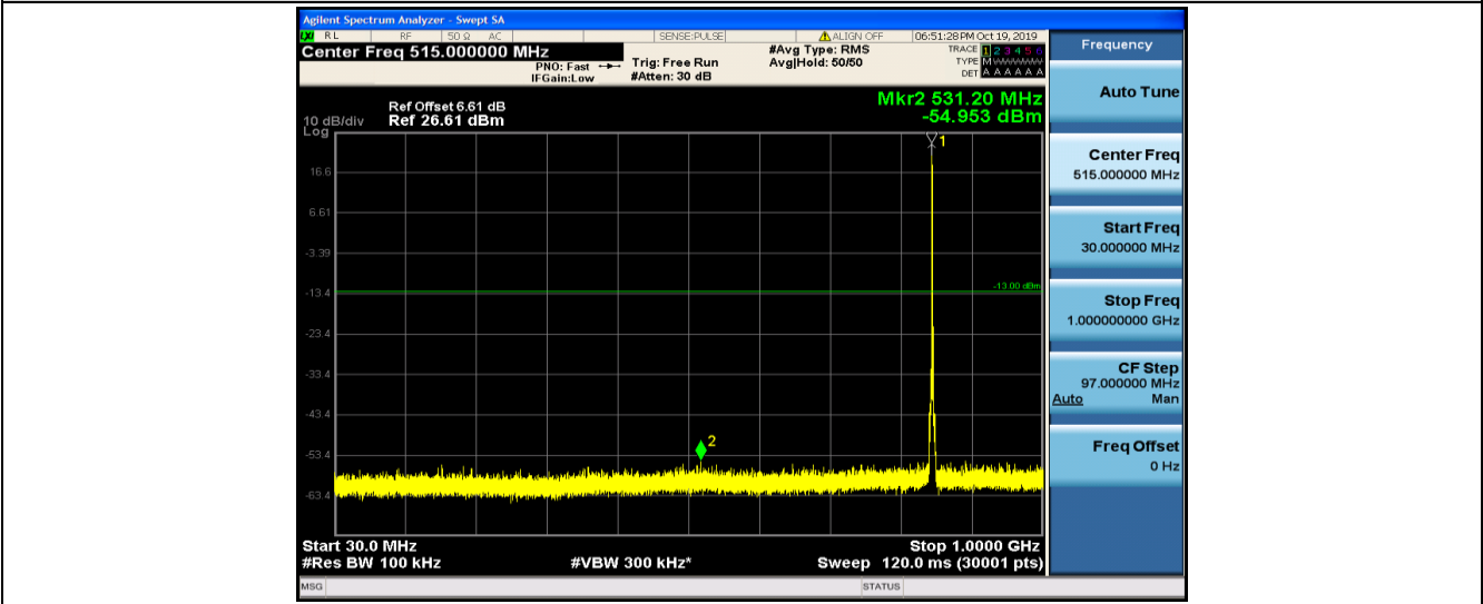
Band5-1.4MHz-QPSK-20643-1RB#0-30~1000MHz
