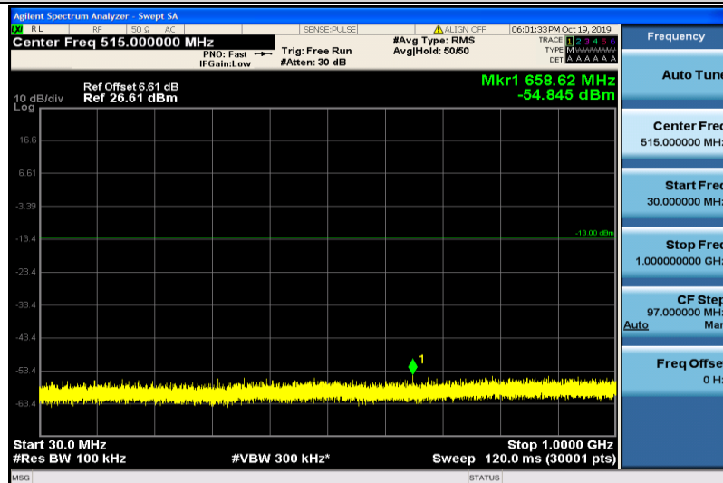
Band4-20MHz-16QAM-20175-1RB#0-30~1000MHz
