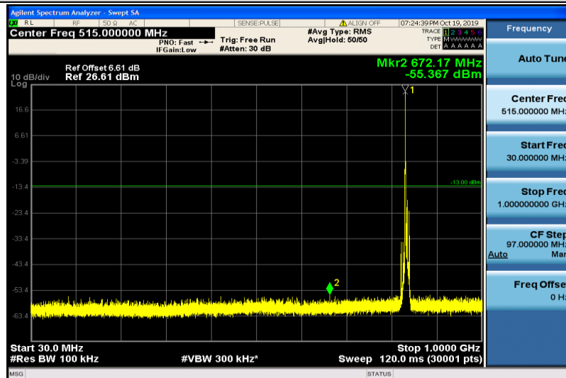
Band5-5MHz-QPSK-20525-1RB#0-30~1000MHz
