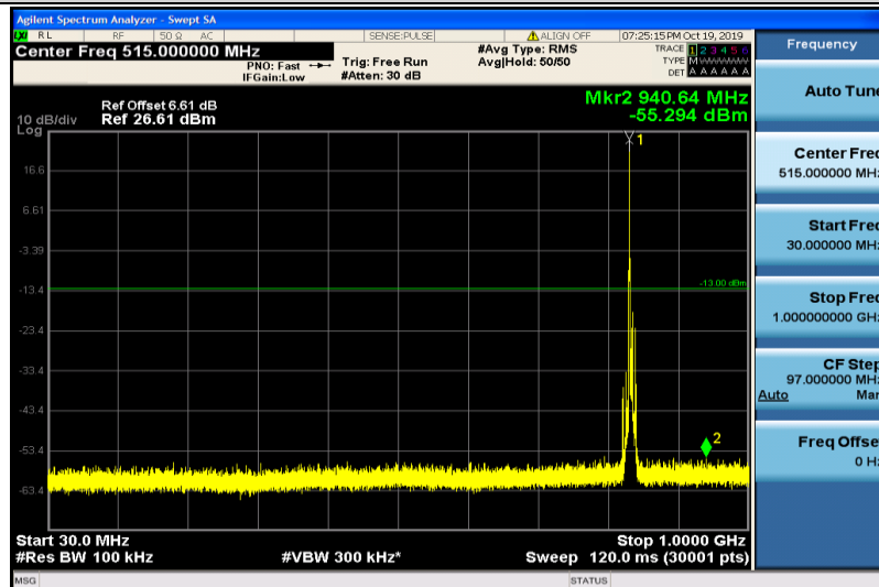
Band5-5MHz-16QAM-20525-1RB#0-30~1000MHz
