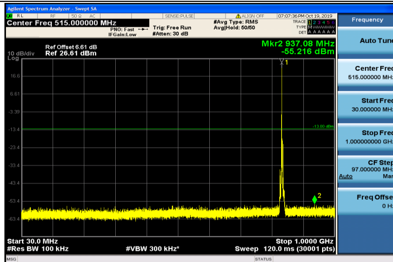
Band5-3MHz-16QAM-20525-1RB#0-30~1000MHz
