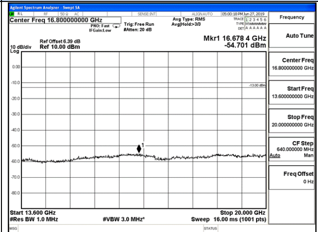
13.6 GHz – 20 GHz
