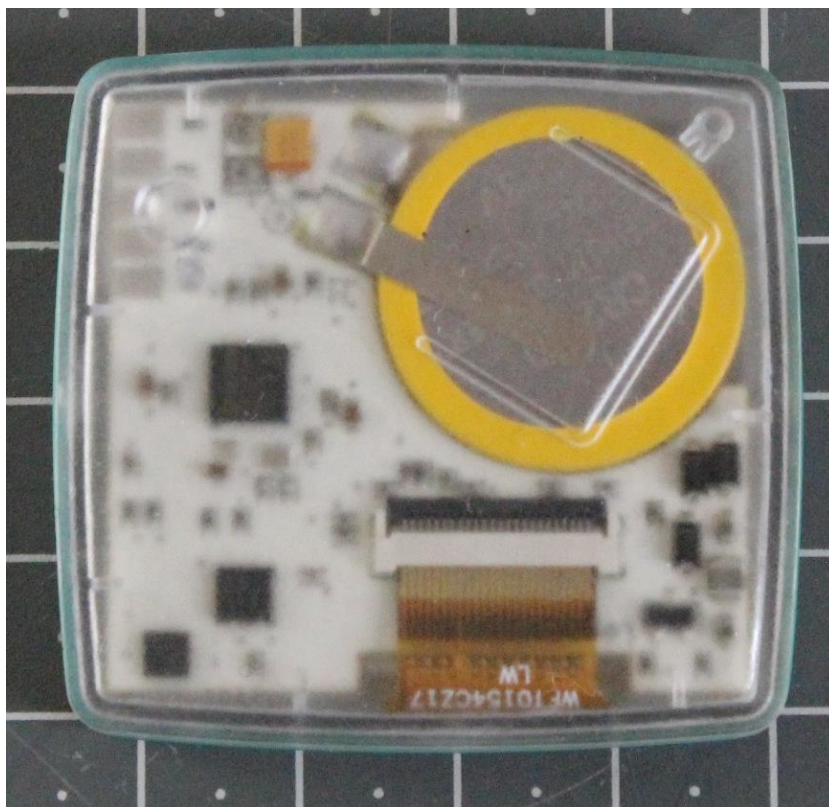
Photograph 2. The EUT (rear side)
