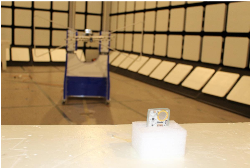
Photograph 3. Radiated emission test setup
