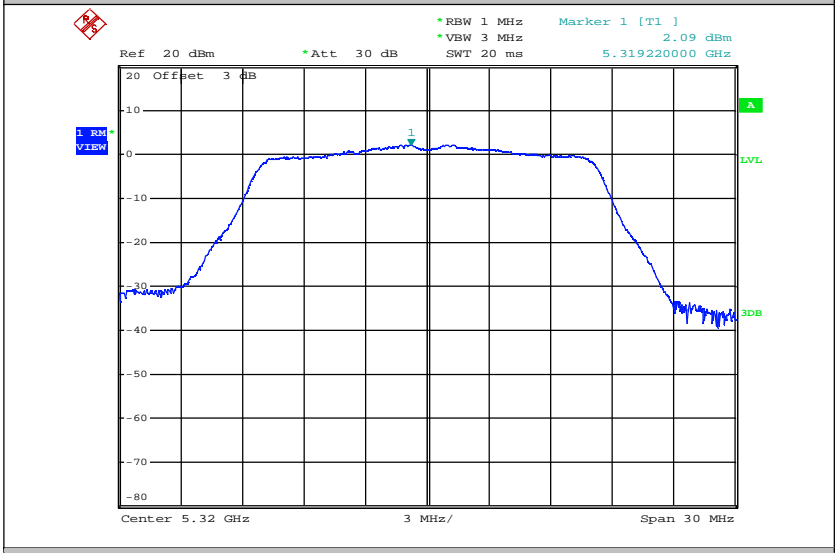
Maximum Power Spectral Density_TNVN_11A_5320_Ant2
