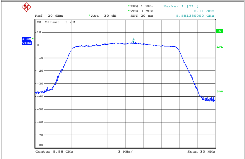
Maximum Power Spectral Density_TNVN_11AC20_5580_Ant2
