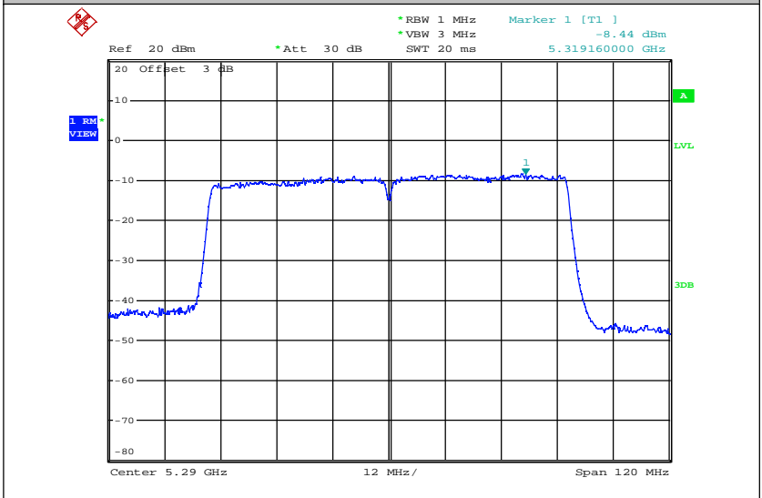
Maximum Power Spectral Density_TNVN_11AC80_5290_Ant2
