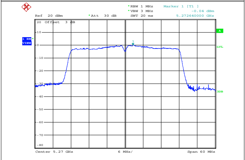
Maximum Power Spectral Density_TNVN_11AC40_5270_Ant2
