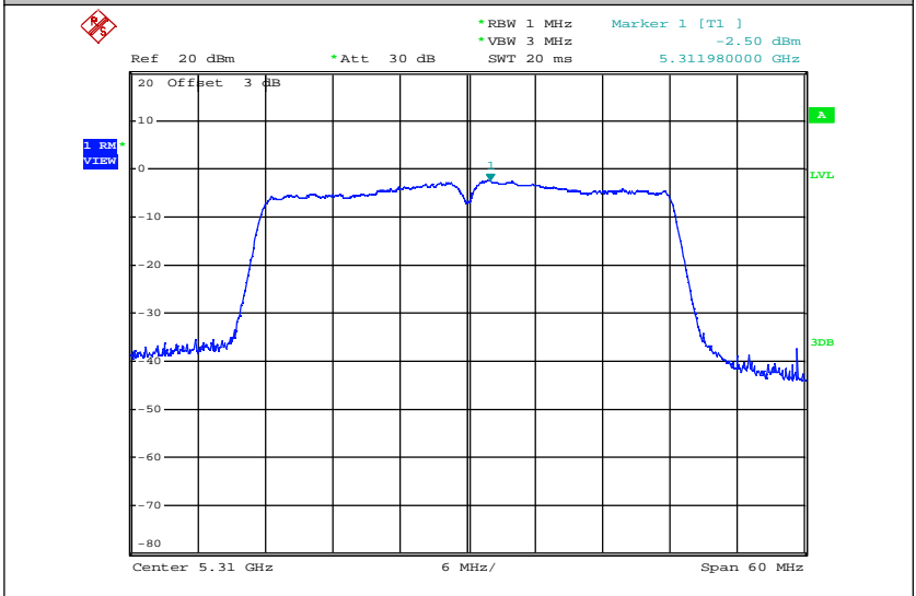
Maximum Power Spectral Density_TNVN_11N40_5310_Ant2
