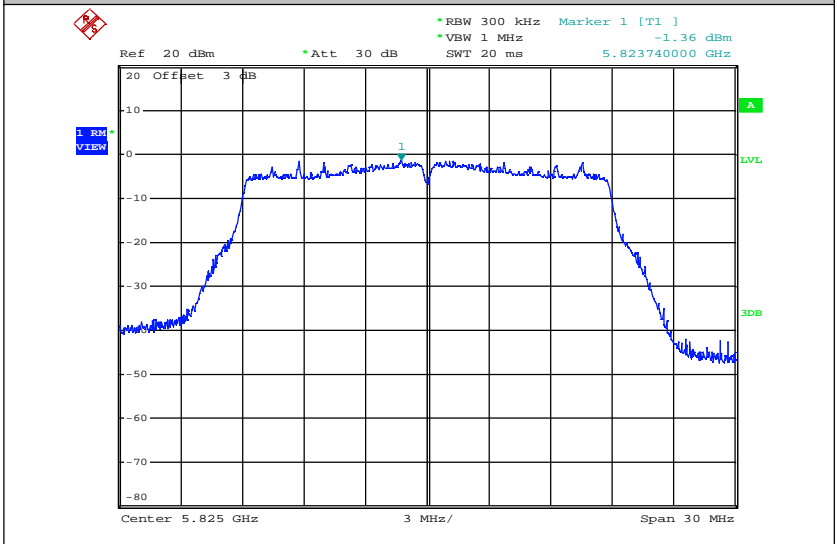
Maximum Power Spectral Density_TNVN_11N20_5825_Ant2
