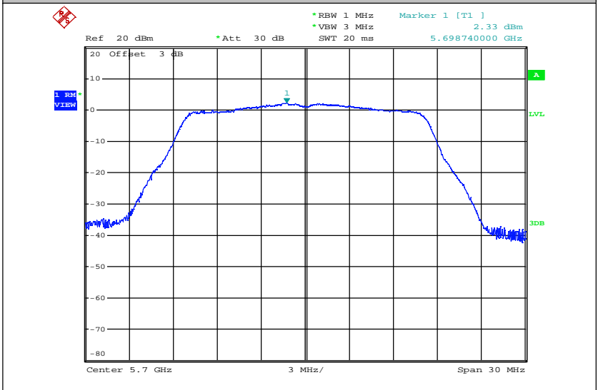
Maximum Power Spectral Density_TNVN_11A_5700_Ant2
