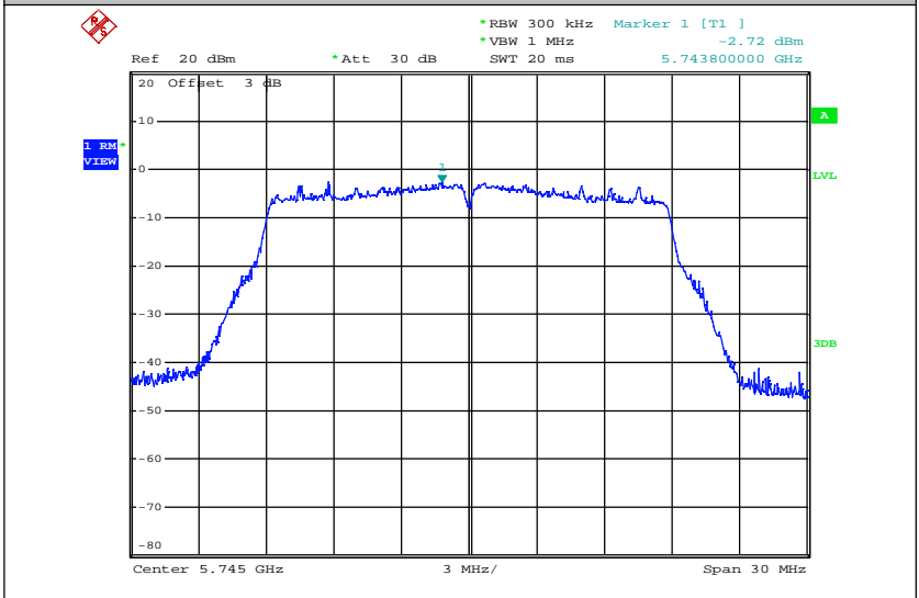
Maximum Power Spectral Density_TNVN_11N20_5745_Ant2
