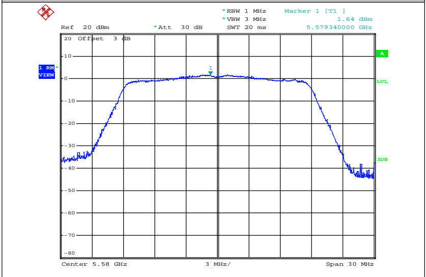
Maximum Power Spectral Density_TNVN_11N20_5580_Ant2
