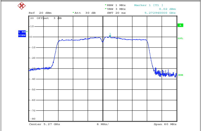
Maximum Power Spectral Density_TNVN_11N40_5270_Ant2
