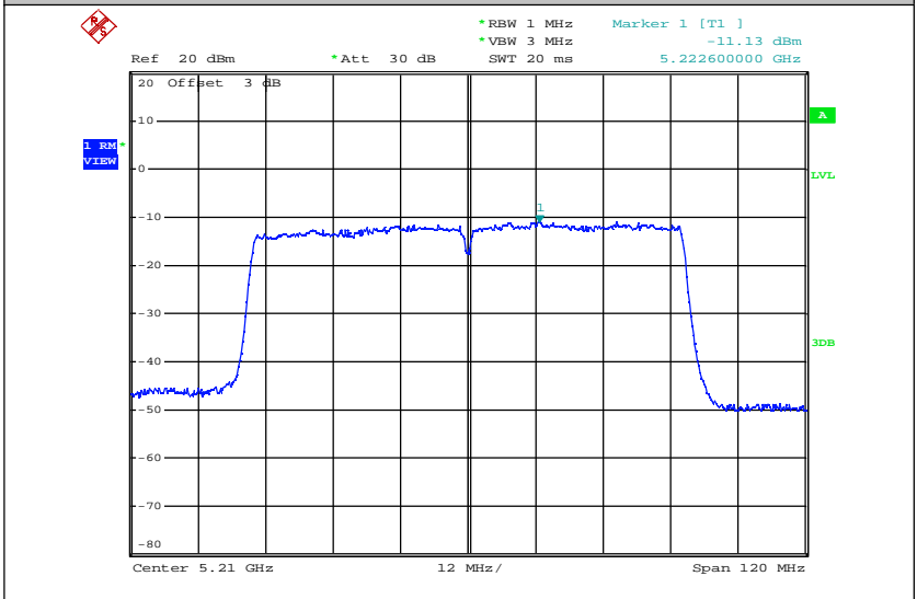
Maximum Power Spectral Density_TNVN_11AC80_5210_Ant2
