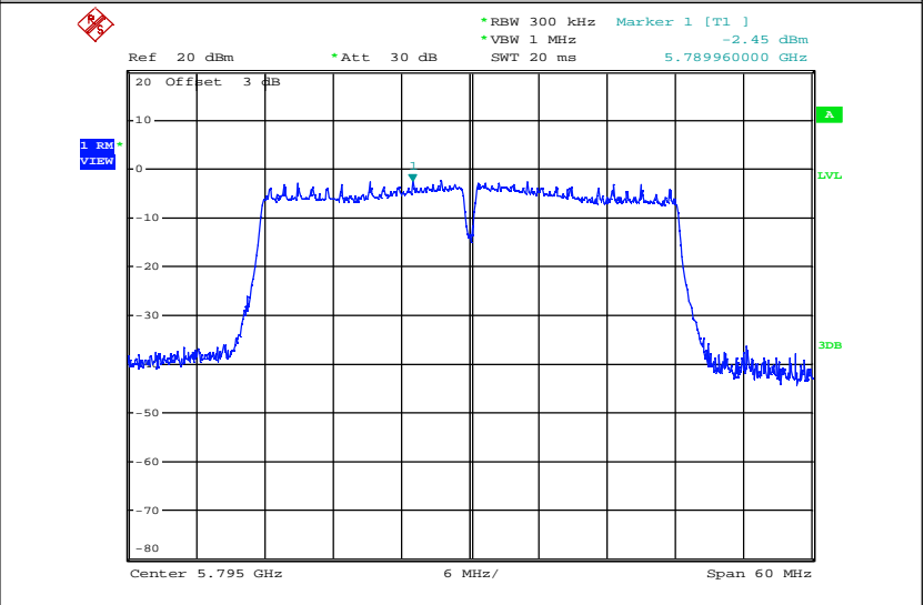
Maximum Power Spectral Density_TNVN_11N40_5795_Ant2
