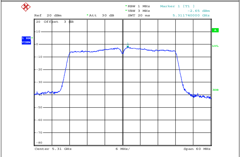
Maximum Power Spectral Density_TNVN_11AC40_5310_Ant2
