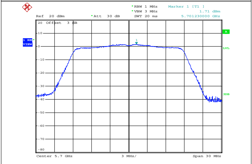
Maximum Power Spectral Density_TNVN_11AC20_5700_Ant2
