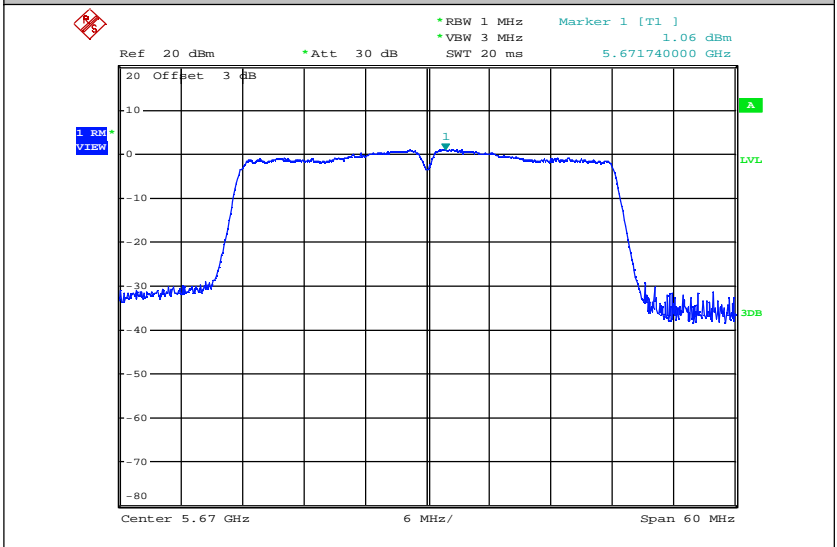
Maximum Power Spectral Density_TNVN_11N40_5670_Ant2
