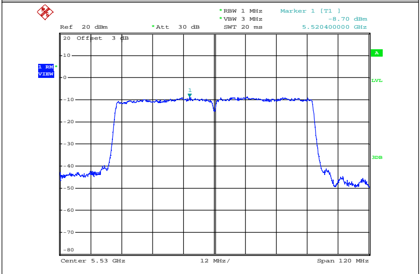
Maximum Power Spectral Density_TNVN_11AC80_5530_Ant2
