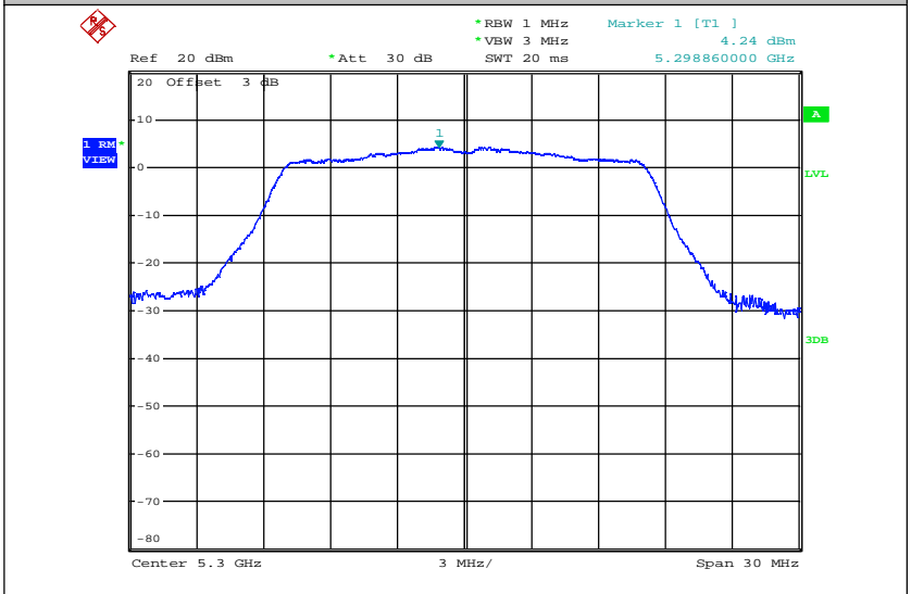
Maximum Power Spectral Density_TNVN_11A_5300_Ant2
