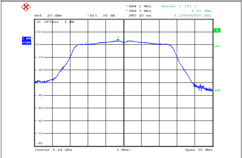
Maximum Power Spectral Density_TNVN_11A_5240_Ant1
