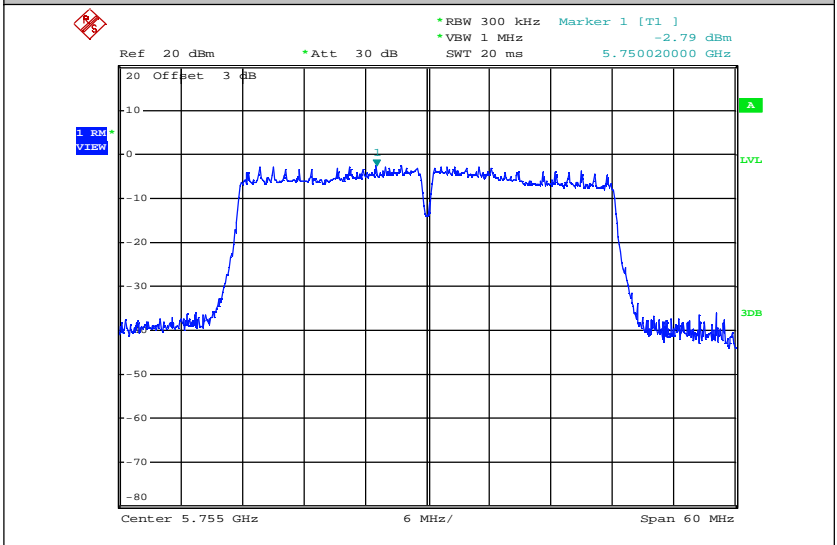
Maximum Power Spectral Density_TNVN_11N40_5755_Ant2
