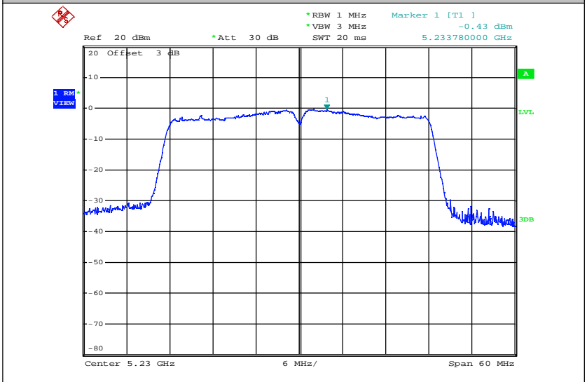
Maximum Power Spectral Density_TNVN_11N40_5230_Ant2
