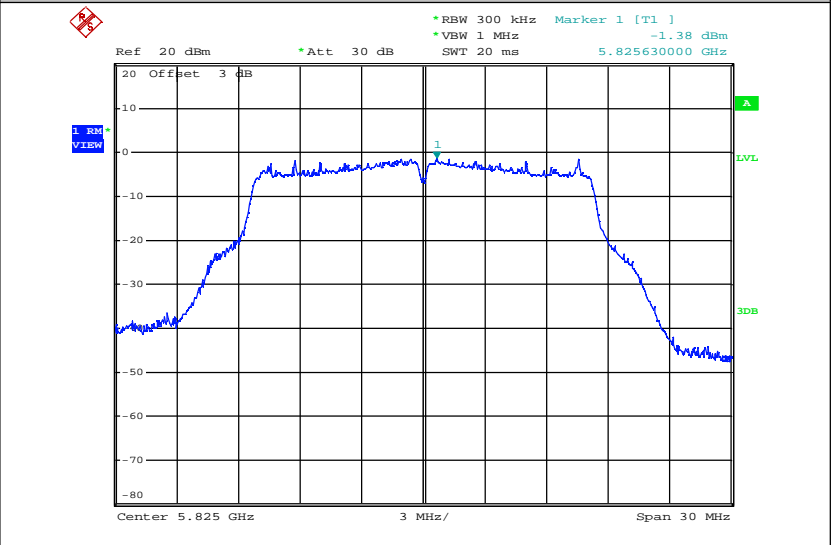
Maximum Power Spectral Density_TNVN_11A_5825_Ant2
