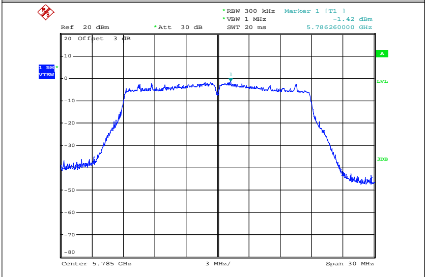
Maximum Power Spectral Density_TNVN_11N20_5785_Ant2
