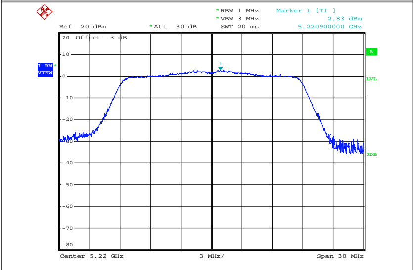
Maximum Power Spectral Density_TNVN_11AC20_5220_Ant2
