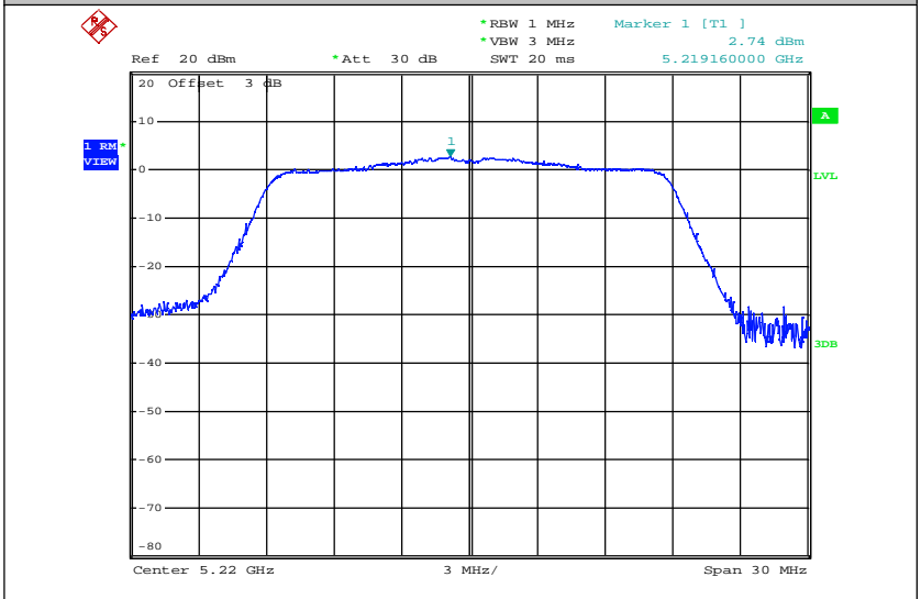
Maximum Power Spectral Density_TNVN_11N20_5220_Ant2
