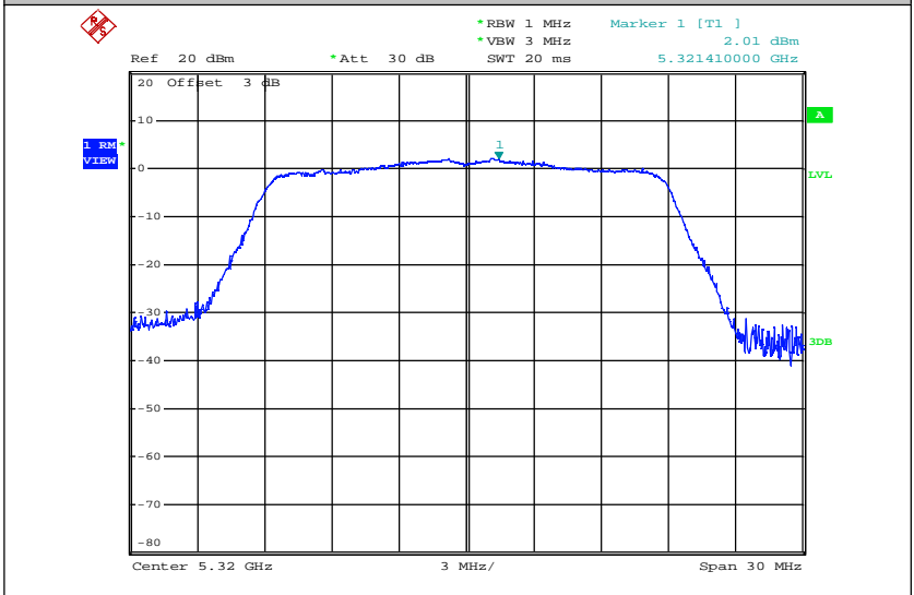
Maximum Power Spectral Density_TNVN_11N20_5320_Ant2
