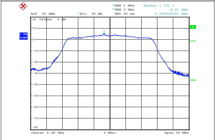
Maximum Power Spectral Density_TNVN_11A_5260_Ant2
