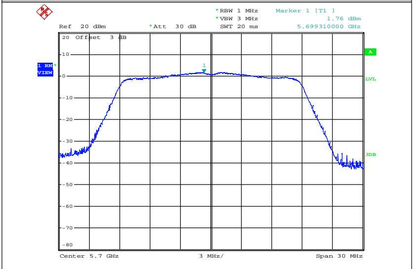
Maximum Power Spectral Density_TNVN_11N20_5700_Ant2
