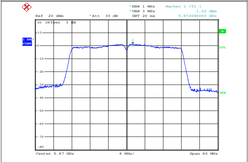
Maximum Power Spectral Density_TNVN_11AC40_5670_Ant2
