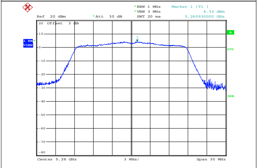
Maximum Power Spectral Density_TNVN_11AC20_5260_Ant2
