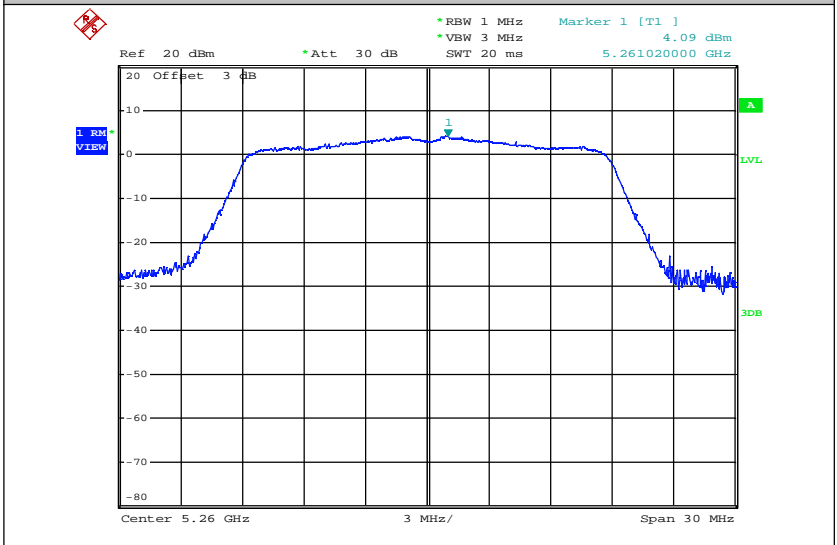
Maximum Power Spectral Density_TNVN_11N20_5260_Ant2
