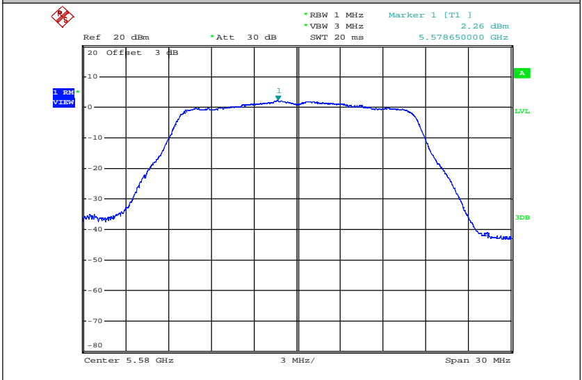
Maximum Power Spectral Density_TNVN_11A_5580_Ant2
