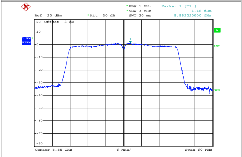
Maximum Power Spectral Density_TNVN_11AC40_5550_Ant2
