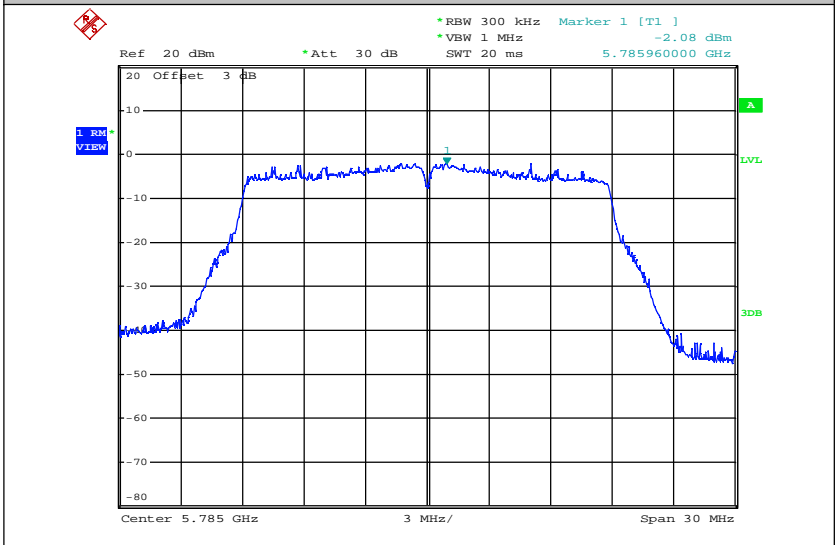
Maximum Power Spectral Density_TNVN_11AC20_5785_Ant2
