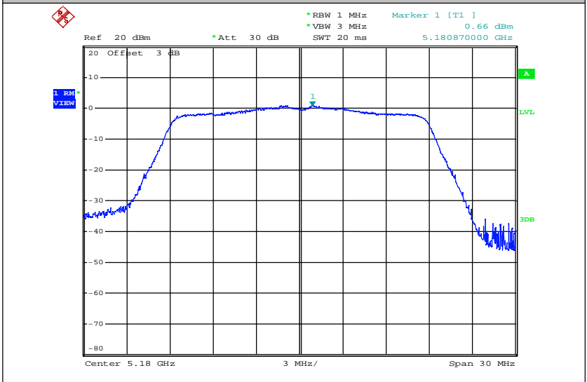
Maximum Power Spectral Density_TNVN_11AC20_5180_Ant2
