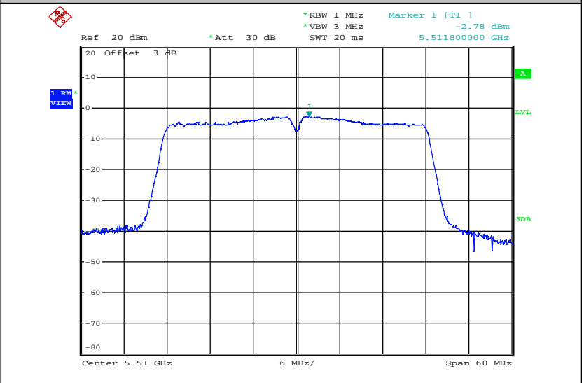
Maximum Power Spectral Density_TNVN_11N40_5510_Ant2
