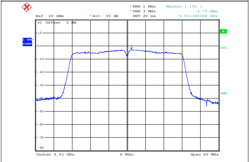
Maximum Power Spectral Density_TNVN_11AC40_5510_Ant2
