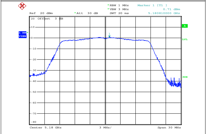
Maximum Power Spectral Density_TNVN_11N20_5180_Ant2
