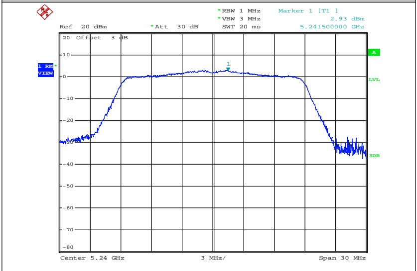
Maximum Power Spectral Density_TNVN_11AC20_5240_Ant2
