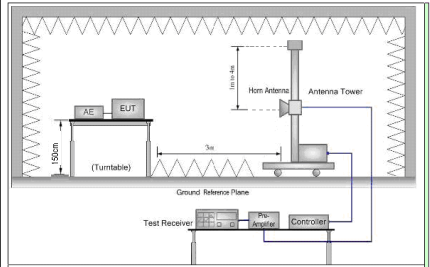
Figure 2. Above 1 GHz
