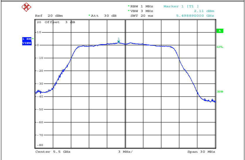
Maximum Power Spectral Density_TNVN_11A_5500_Ant2
