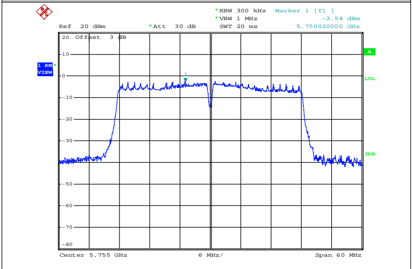
Maximum Power Spectral Density_TNVN_11AC40_5755_Ant2
