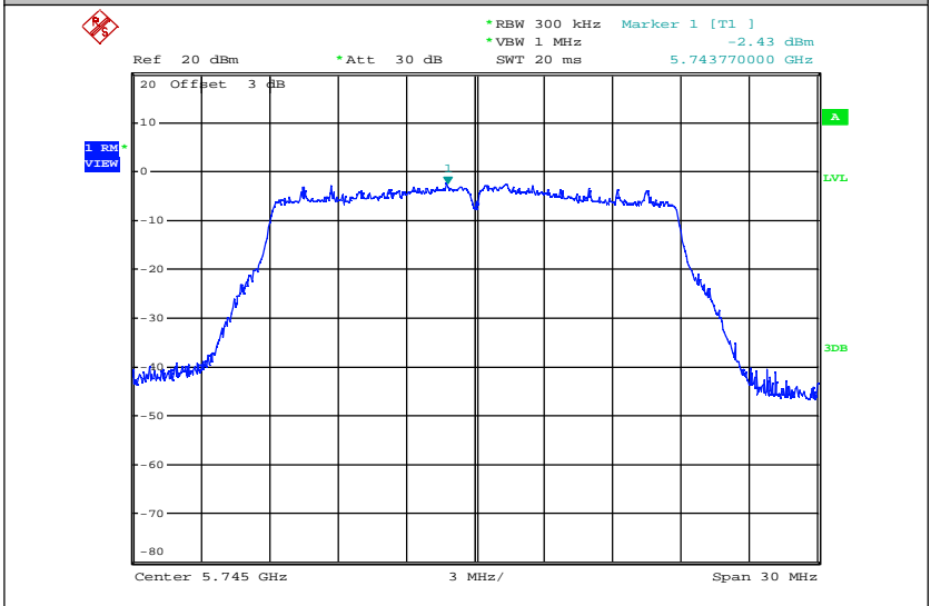
Maximum Power Spectral Density_TNVN_11AC20_5745_Ant2
