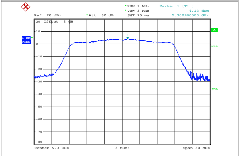
Maximum Power Spectral Density_TNVN_11AC20_5300_Ant2
