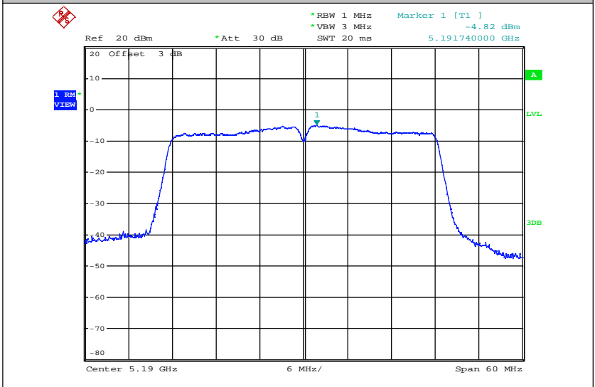
Maximum Power Spectral Density_TNVN_11N40_5190_Ant2
