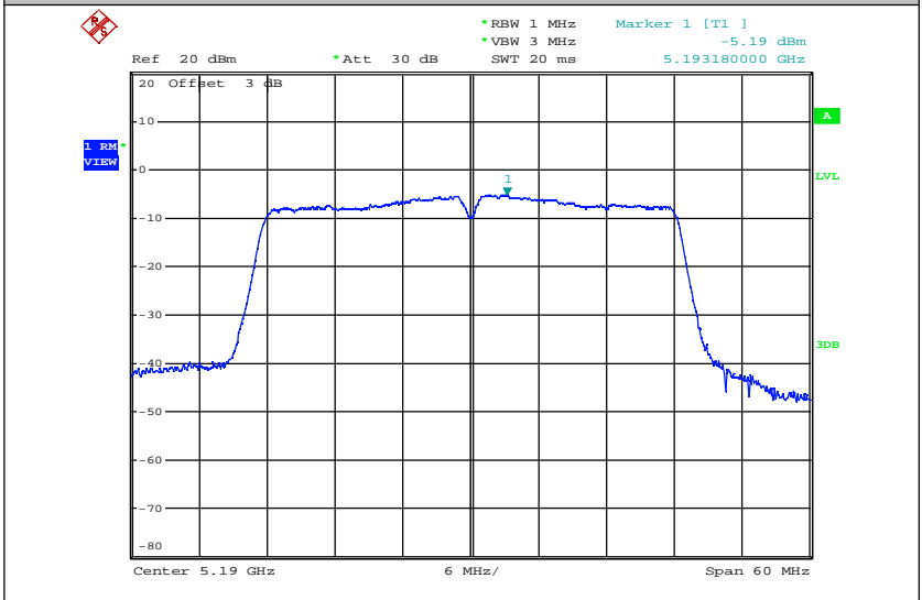
Maximum Power Spectral Density_TNVN_11AC40_5190_Ant2
