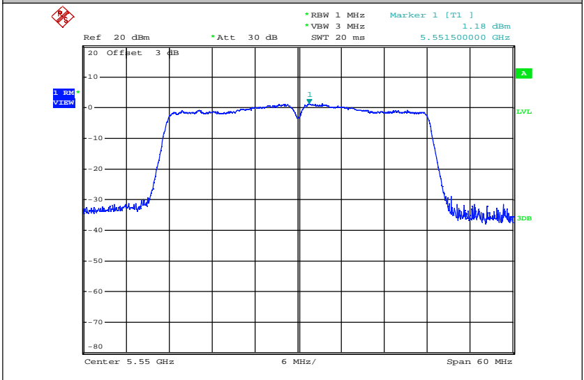
Maximum Power Spectral Density_TNVN_11N40_5550_Ant2
