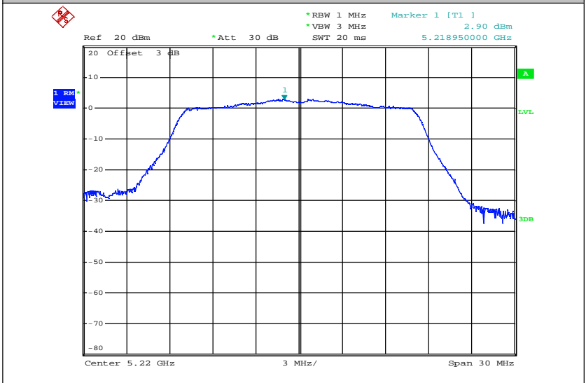
Maximum Power Spectral Density_TNVN_11A_5220_Ant2
