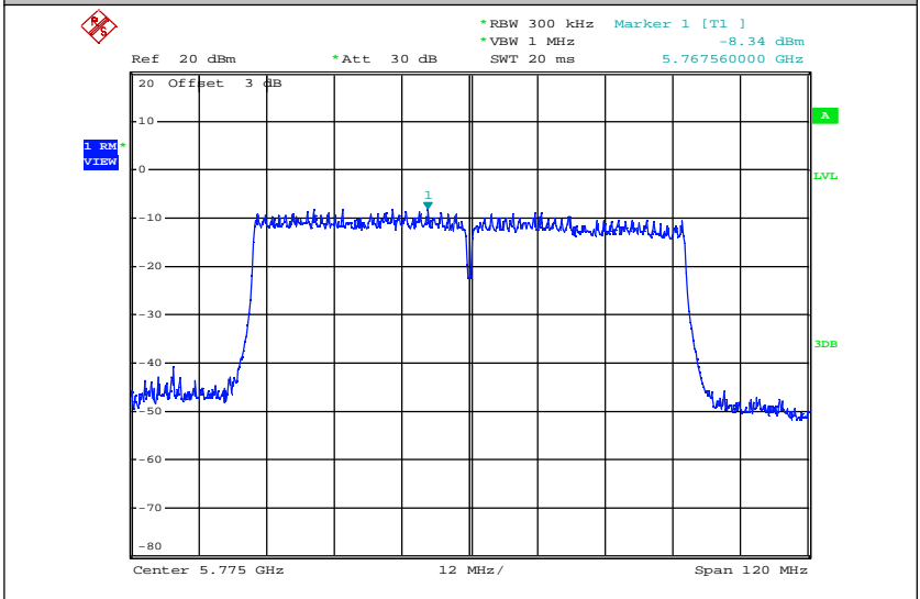
Maximum Power Spectral Density_TNVN_11AC80_5775_Ant2
