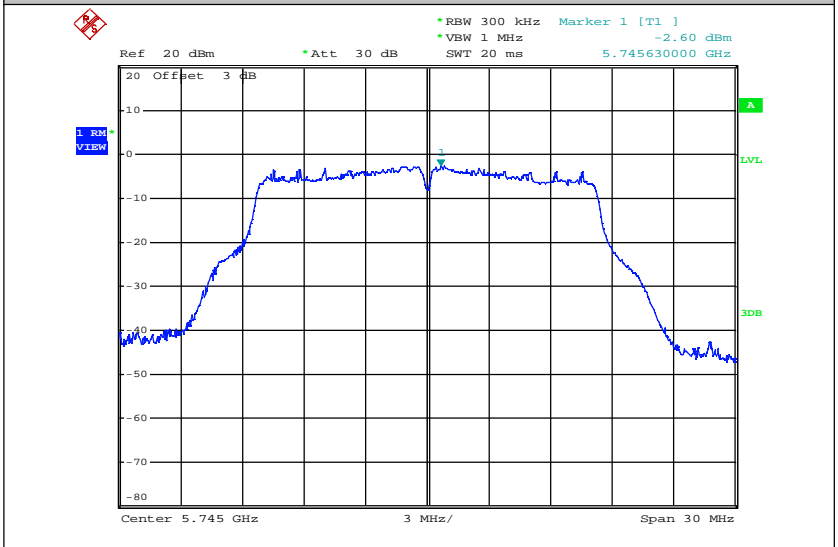
Maximum Power Spectral Density_TNVN_11A_5745_Ant2
