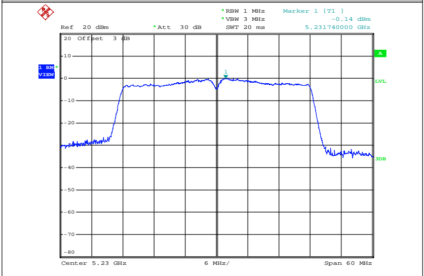
Maximum Power Spectral Density_TNVN_11AC40_5230_Ant2
