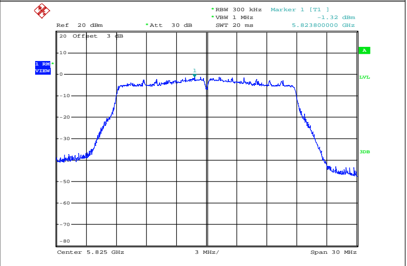
Maximum Power Spectral Density_TNVN_11AC20_5825_Ant2
