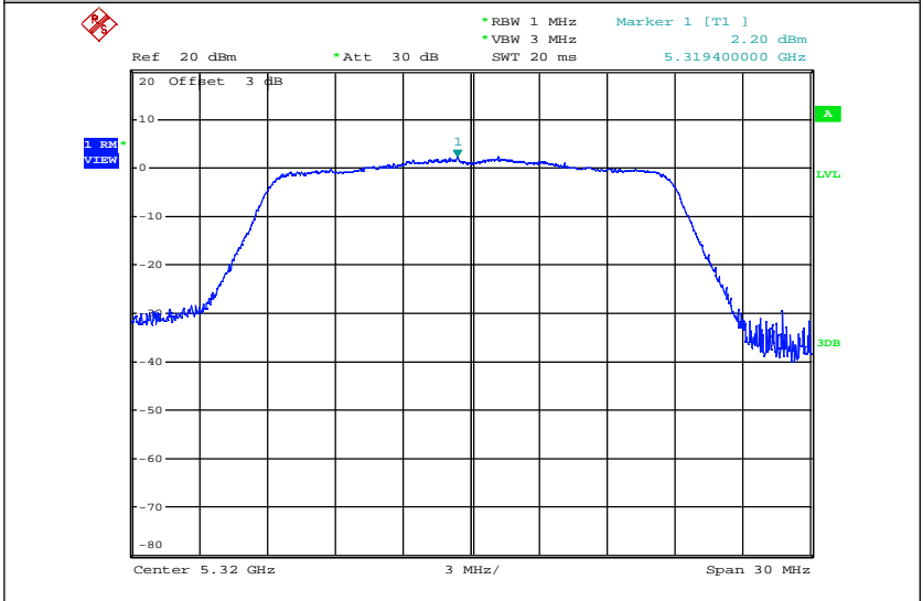
Maximum Power Spectral Density_TNVN_11AC20_5320_Ant2
