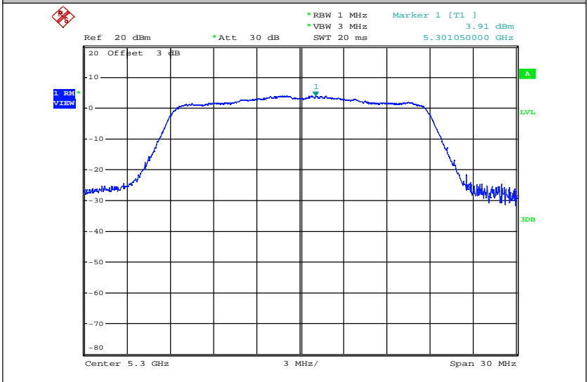
Maximum Power Spectral Density_TNVN_11N20_5300_Ant2
