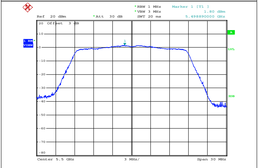
Maximum Power Spectral Density_TNVN_11AC20_5500_Ant2
