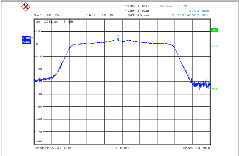
Maximum Power Spectral Density_TNVN_11N20_5240_Ant2
