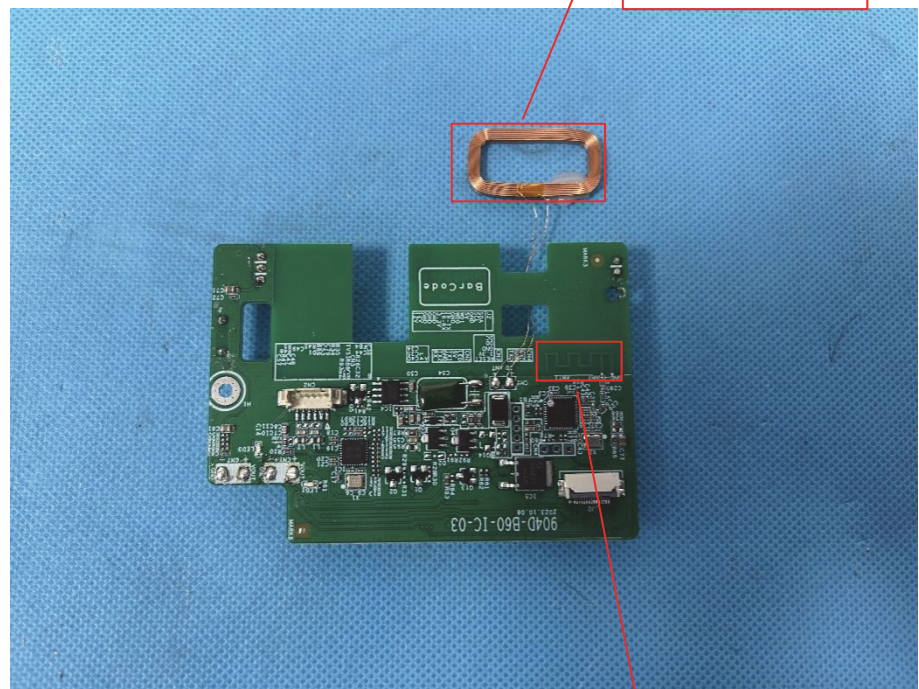
125 kHz Antenna
