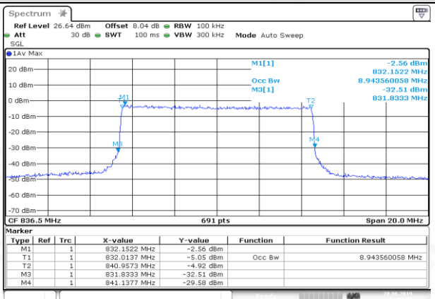
MCH_16QAM_50RB#0
