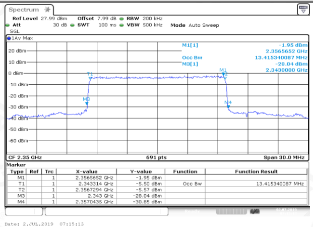
MCH_16QAM_75RB#0
