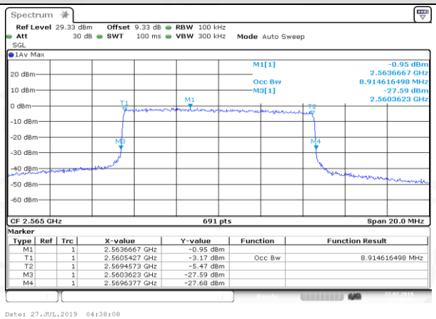
HCH_16QAM_50RB#0
