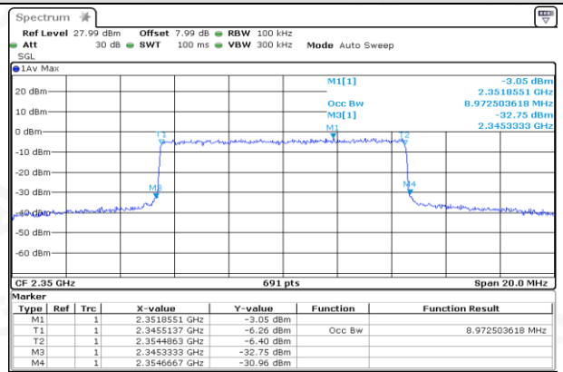
MCH_16QAM_50RB#0
