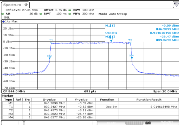
HCH_QPSK_50RB#0
