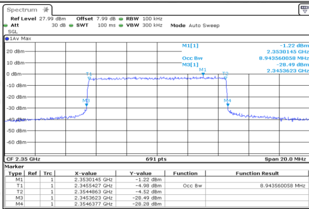
MCH_QPSK_50RB#0
