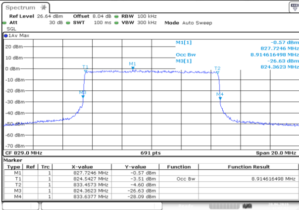
LCH_QPSK_50RB#0
