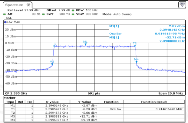
HCH_16QAM_50RB#0
