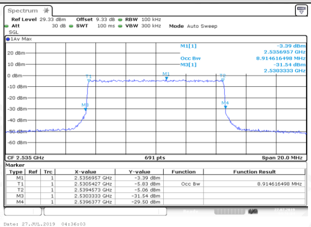
MCH_16QAM_50RB#0
