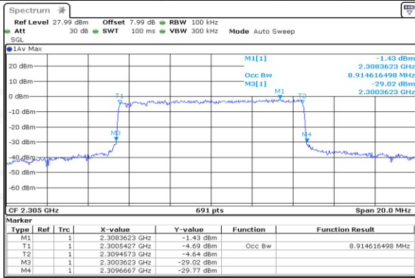
LCH_QPSK_50RB#0
