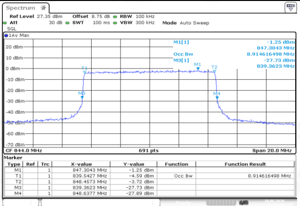
HCH_16QAM_50RB#0
