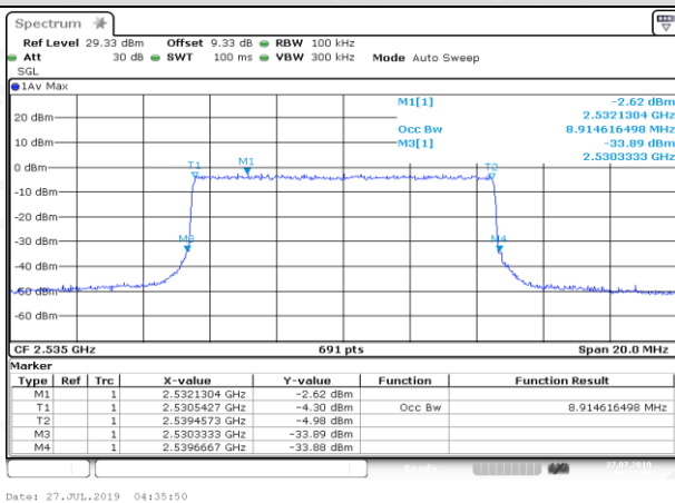
MCH_QPSK_50RB#0
