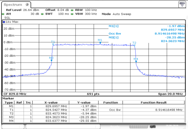
LCH_16QAM_50RB#0
