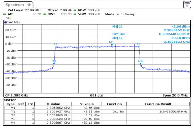
LCH_16QAM_50RB#0
