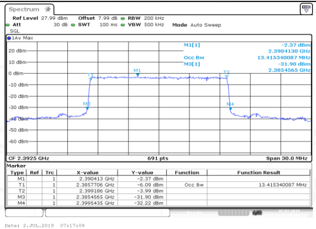
HCH_16QAM_75RB#0
