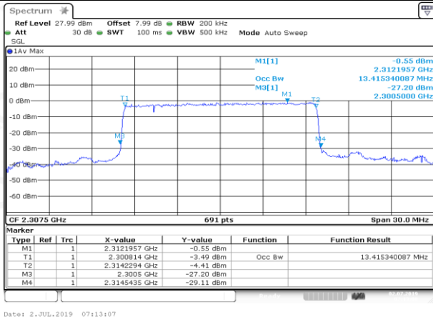
LCH_QPSK_75RB#0
