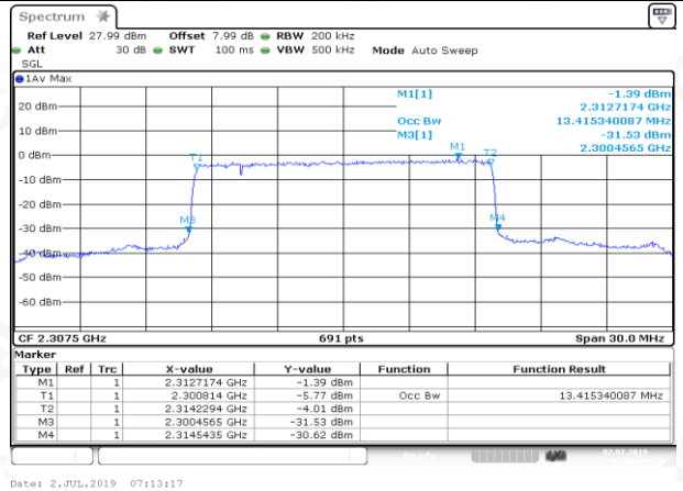
LCH_16QAM_75RB#0
