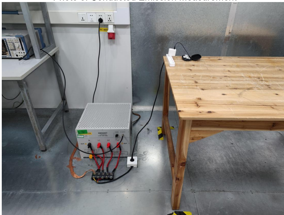
FCC ID: 2ATS9-1314 Photo of Conducted Emission Measurement
