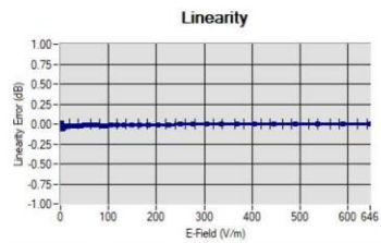
Linearity: +/-1.35% (+/-0.06dB)
