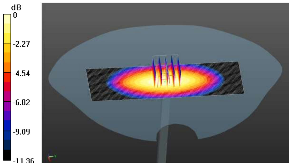
0 dB = 1.06 W/kg = 0.25 dBW/kg
