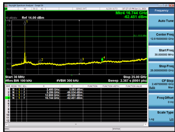
Mode 2 CH39(2480MHz)
