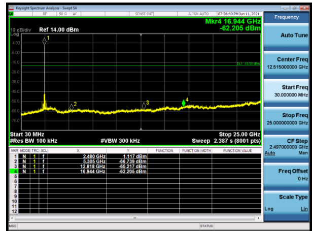
Mode 4 CH39(2480MHz)
