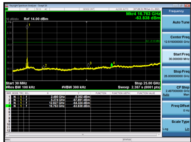
Mode 2 CH39(2480MHz)
