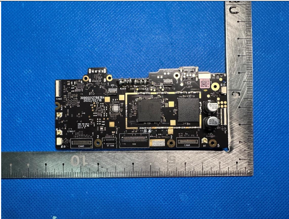
EUT Photo(8) Wi-Fi Chip
