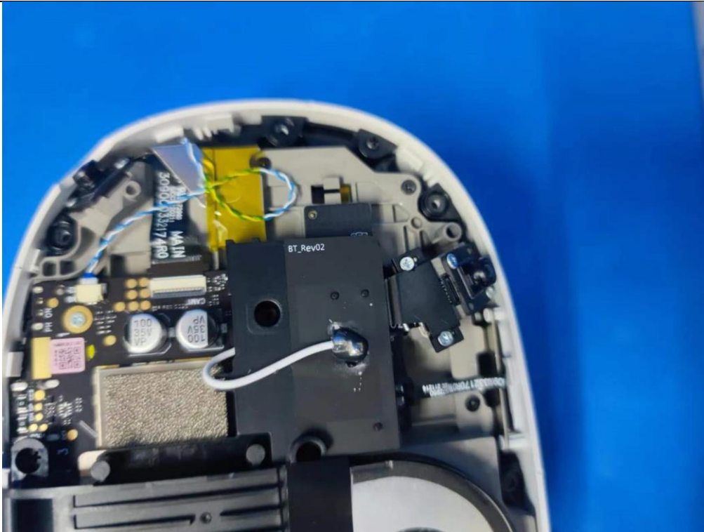
EUT Photo(4) Wifi Antenna1
