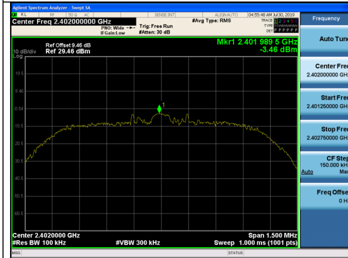
\pi/4 -DQPSK on Channel 00
