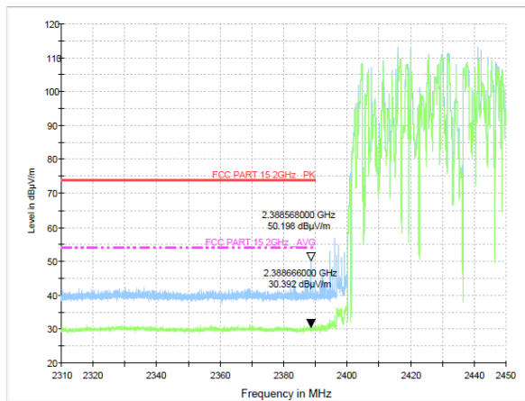
Test Mode: GFSK-Low Hopping-on Polarization: Vertical
