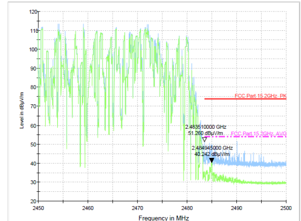
Test Mode: GFSK-High Hopping-on Polarization: Horizontal
