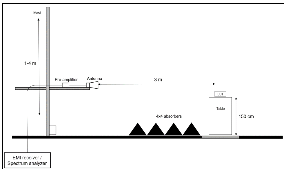
Figure 64. Test setup.
