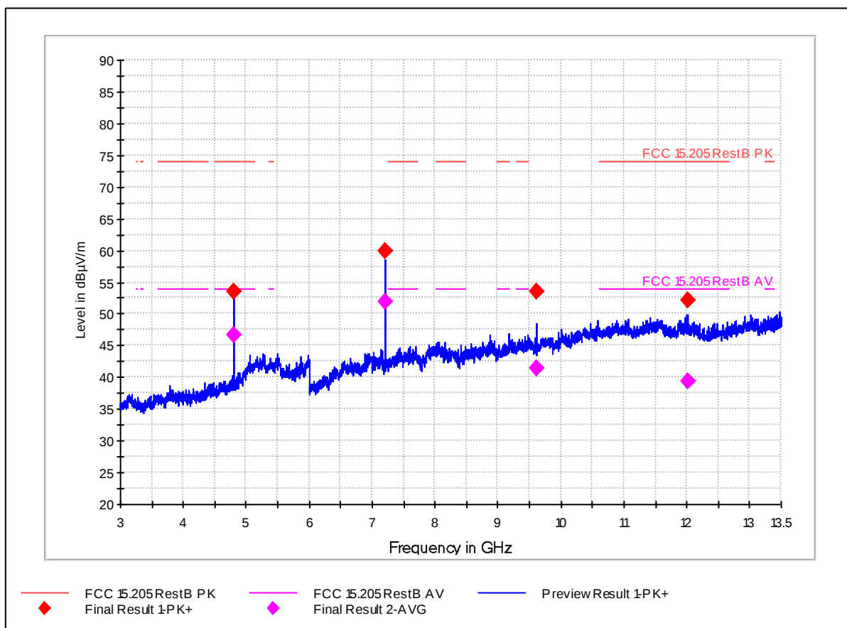
Figure 49. Radiated emission test results 3 – 13.5 GHz. EUT ver.
