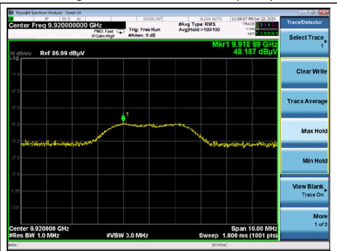
High channel 4 th Harmonics (Peak)
