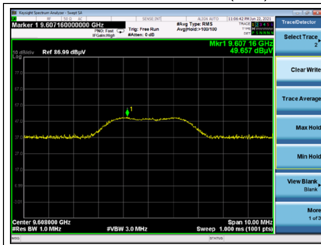
Low channel 4 th Harmonics (Peak)
