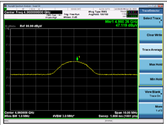
High channel 2 nd Harmonics (Average)
