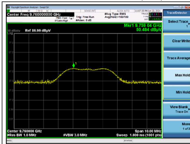
Middle channel 4 th Harmonics (Peak)
